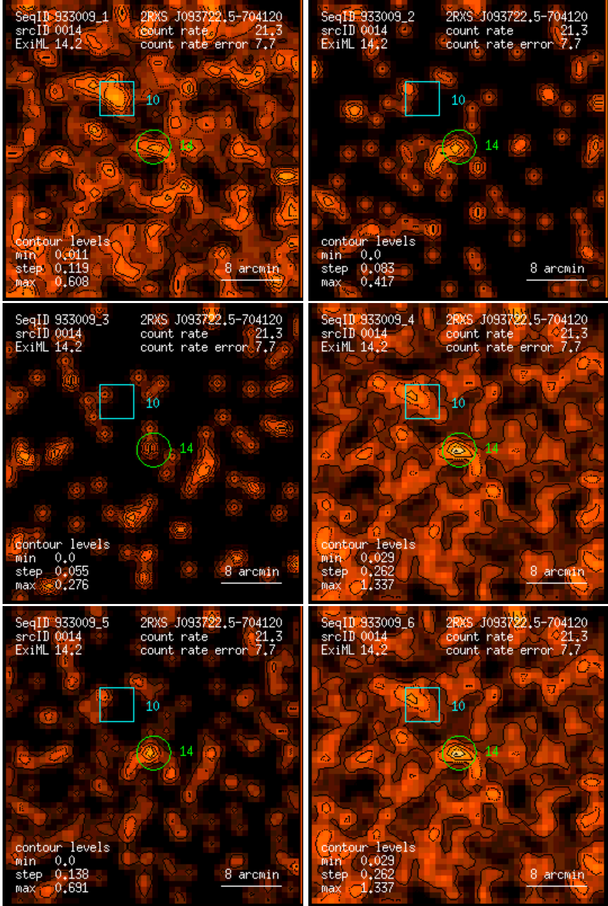
Figure 14: RASS 933009: detection 0014: band rate images, Gaussian filter: (1) PSPC channels 11 – 41, (2) 52 – 90, (3) 91 – 201, (4) 11 – 235, (5) 52 – 201, (6) 11 – 201. Broad band rates in counts/ks. Band rate contour levels in counts/ks/arcmin 2 .
