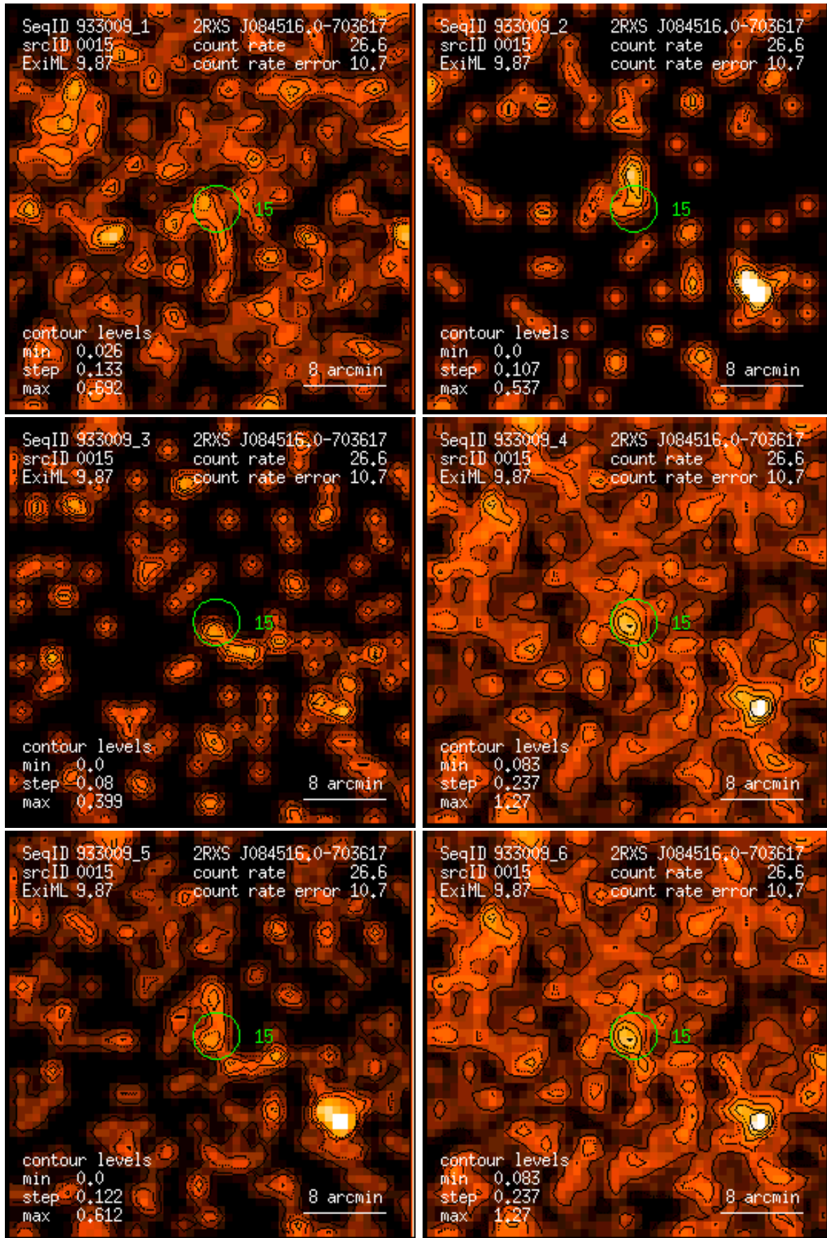
Figure 15: RASS 933009: detection 0015: band rate images, Gaussian filter: (1) PSPC channels 11 – 41, (2) 52 – 90, (3) 91 – 201, (4) 11 – 235, (5) 52 – 201, (6) 11 – 201. Broad band rates in counts/ks. Band rate contour levels in counts/ks/arcmin 2 .
