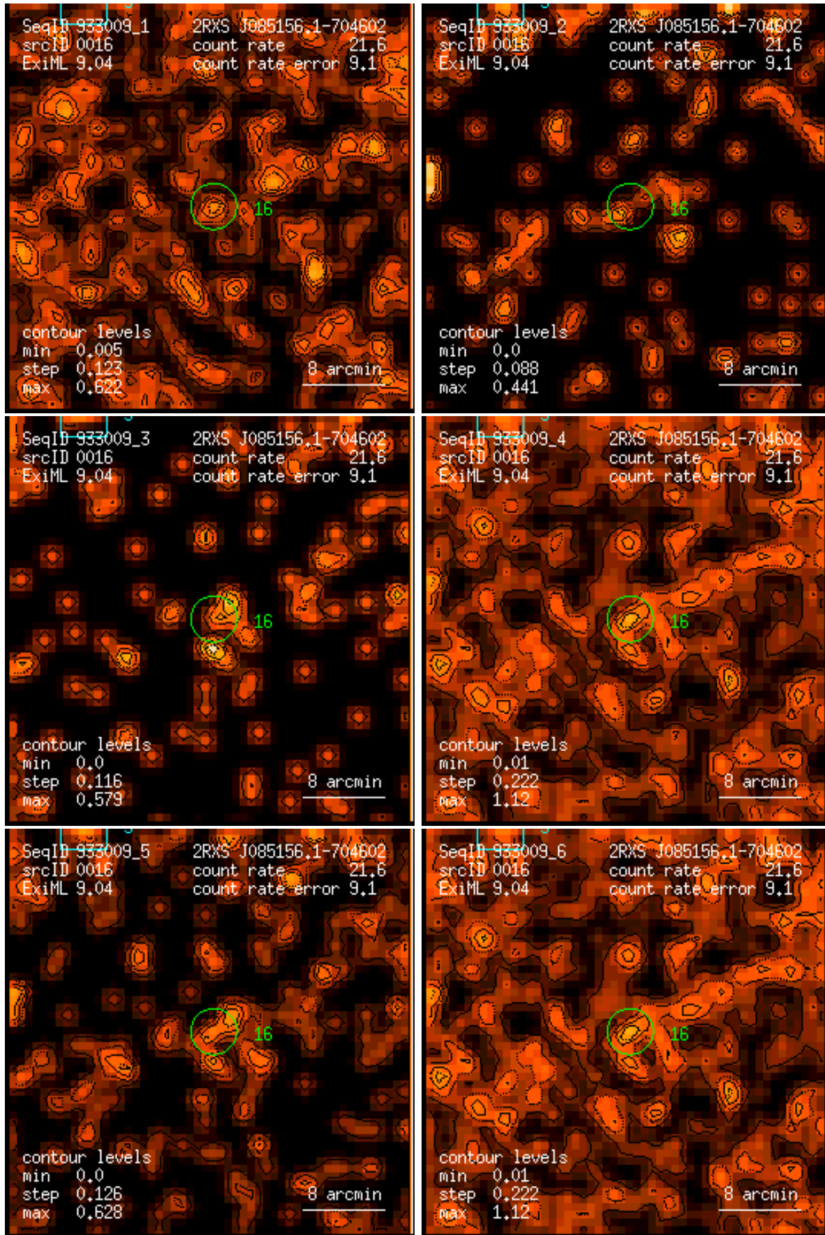
Figure 16: RASS 933009: detection 0016: band rate images, Gaussian filter: (1) PSPC channels 11 – 41, (2) 52 – 90, (3) 91 – 201, (4) 11 – 235, (5) 52 – 201, (6) 11 – 201. Broad band rates in counts/ks. Band rate contour levels in counts/ks/arcmin 2 .
