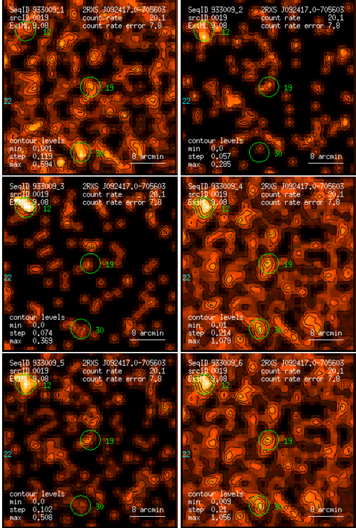
Figure 19: RASS 933009: detection 0019: band rate images, Gaussian filter: (1) PSPC channels 11 – 41, (2) 52 – 90, (3) 91 – 201, (4) 11 – 235, (5) 52 – 201, (6) 11 – 201. Broad band rates in counts/ks. Band rate contour levels in counts/ks/arcmin 2 .
