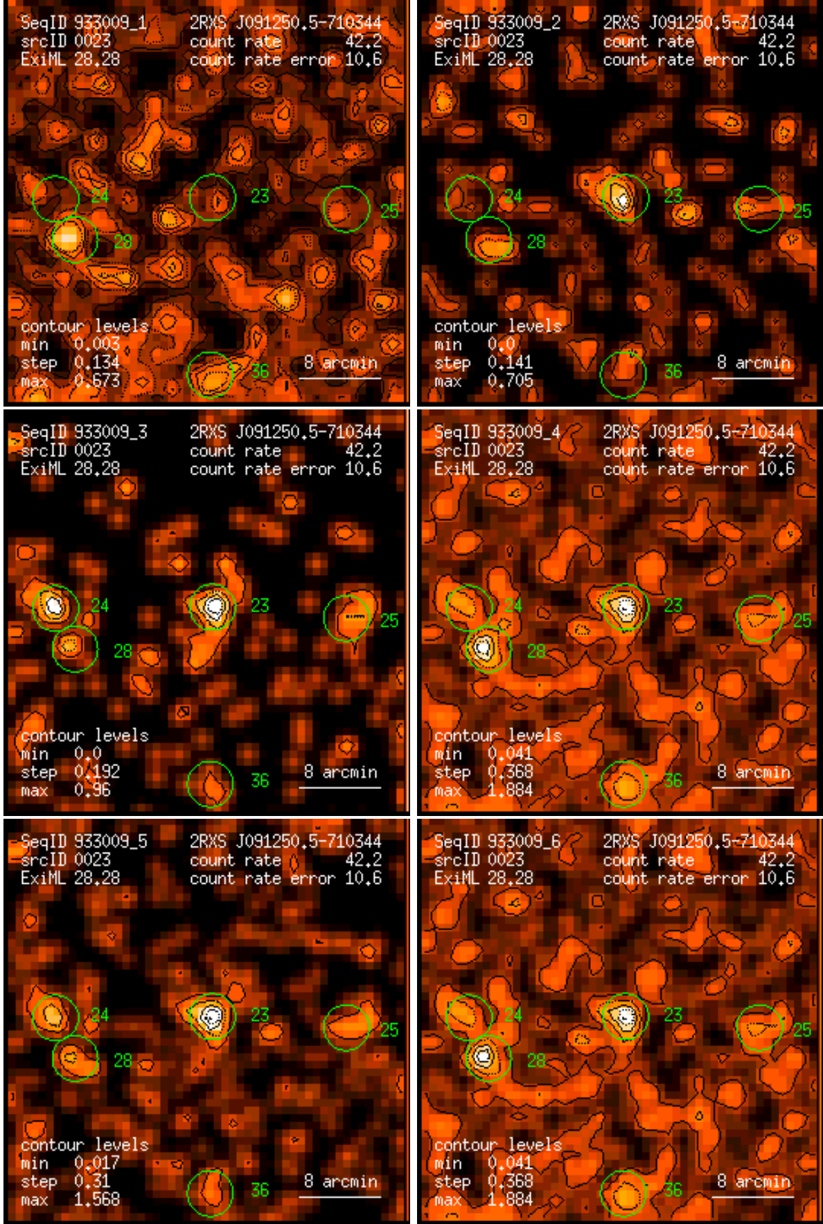
Figure 23: RASS 933009: detection 0023: band rate images, Gaussian filter: (1) PSPC channels 11 – 41, (2) 52 – 90, (3) 91 – 201, (4) 11 – 235, (5) 52 – 201, (6) 11 – 201. Broad band rates in counts/ks. Band rate contour levels in counts/ks/arcmin 2 .
