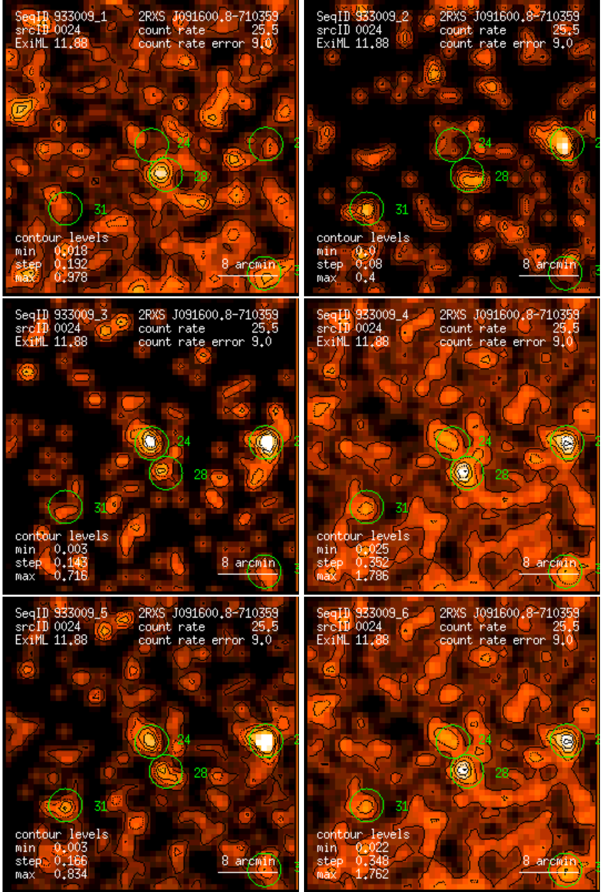
Figure 24: RASS 933009: detection 0024: band rate images, Gaussian filter: (1) PSPC channels 11 – 41, (2) 52 – 90, (3) 91 – 201, (4) 11 – 235, (5) 52 – 201, (6) 11 – 201. Broad band rates in counts/ks. Band rate contour levels in counts/ks/arcmin 2 .
