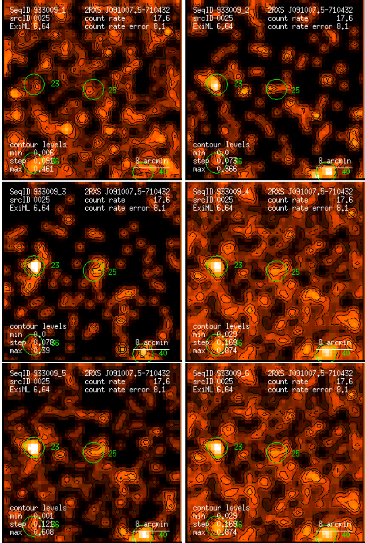
Figure 25: RASS 933009: detection 0025: band rate images, Gaussian filter: (1) PSPC channels 11 – 41, (2) 52 – 90, (3) 91 – 201, (4) 11 – 235, (5) 52 – 201, (6) 11 – 201. Broad band rates in counts/ks. Band rate contour levels in counts/ks/arcmin 2 .
