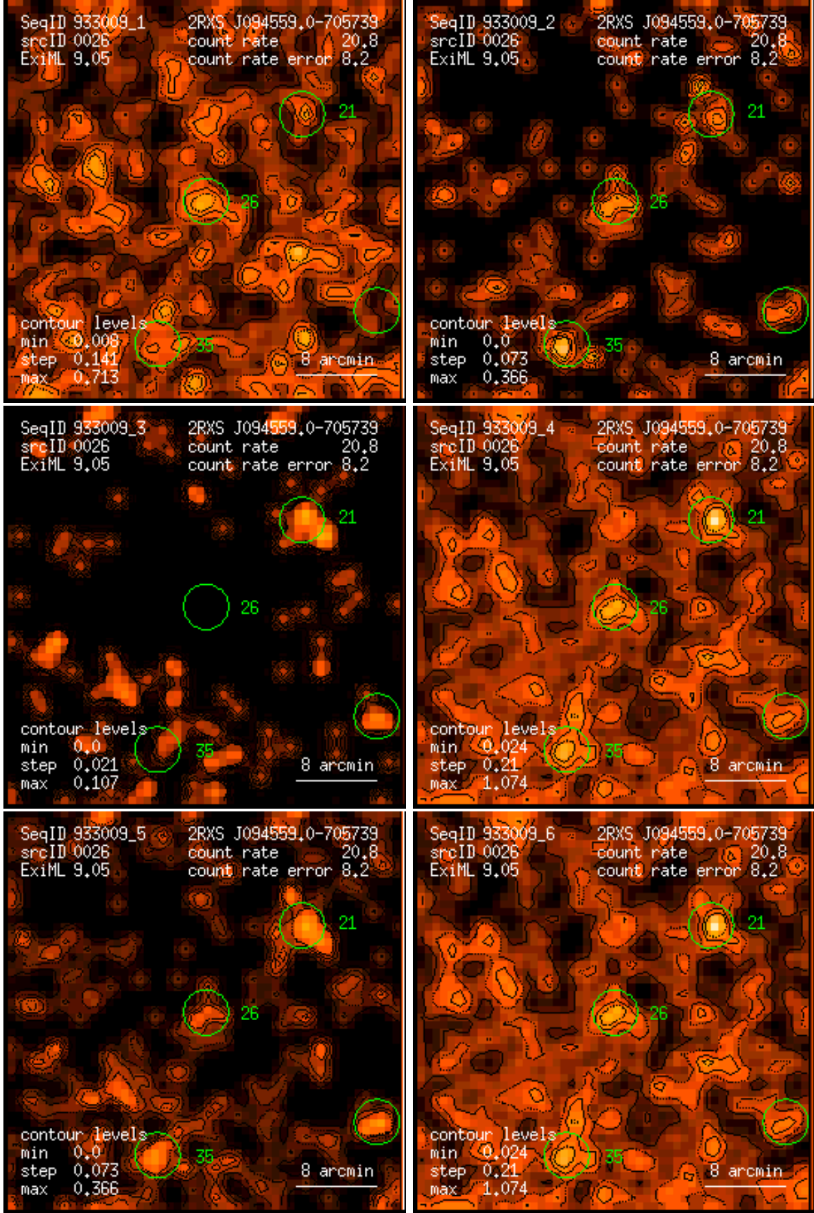
Figure 26: RASS 933009: detection 0026: band rate images, Gaussian filter: (1) PSPC channels 11 – 41, (2) 52 – 90, (3) 91 – 201, (4) 11 – 235, (5) 52 – 201, (6) 11 – 201. Broad band rates in counts/ks. Band rate contour levels in counts/ks/arcmin 2 .
