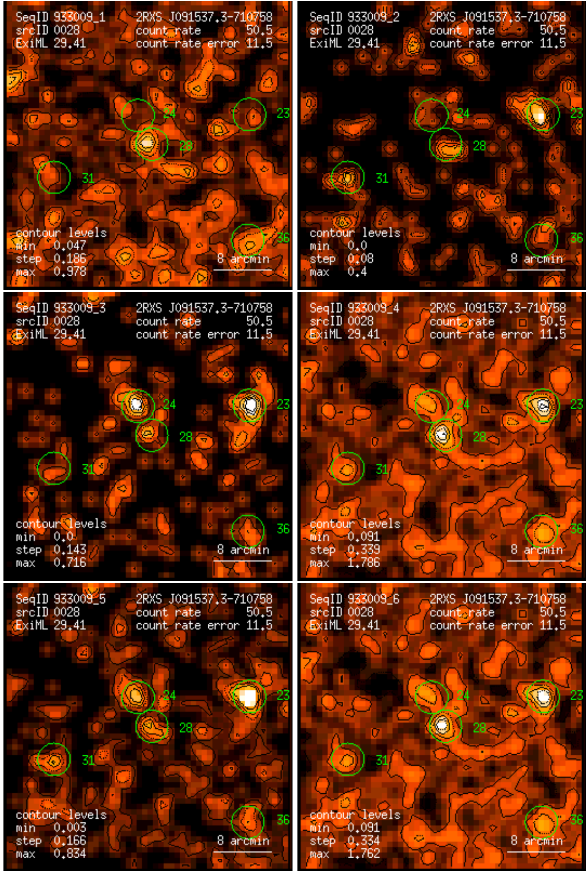
Figure 28: RASS 933009: detection 0028: band rate images, Gaussian filter: (1) PSPC channels 11 – 41, (2) 52 – 90, (3) 91 – 201, (4) 11 – 235, (5) 52 – 201, (6) 11 – 201. Broad band rates in counts/ks. Band rate contour levels in counts/ks/arcmin 2 .
