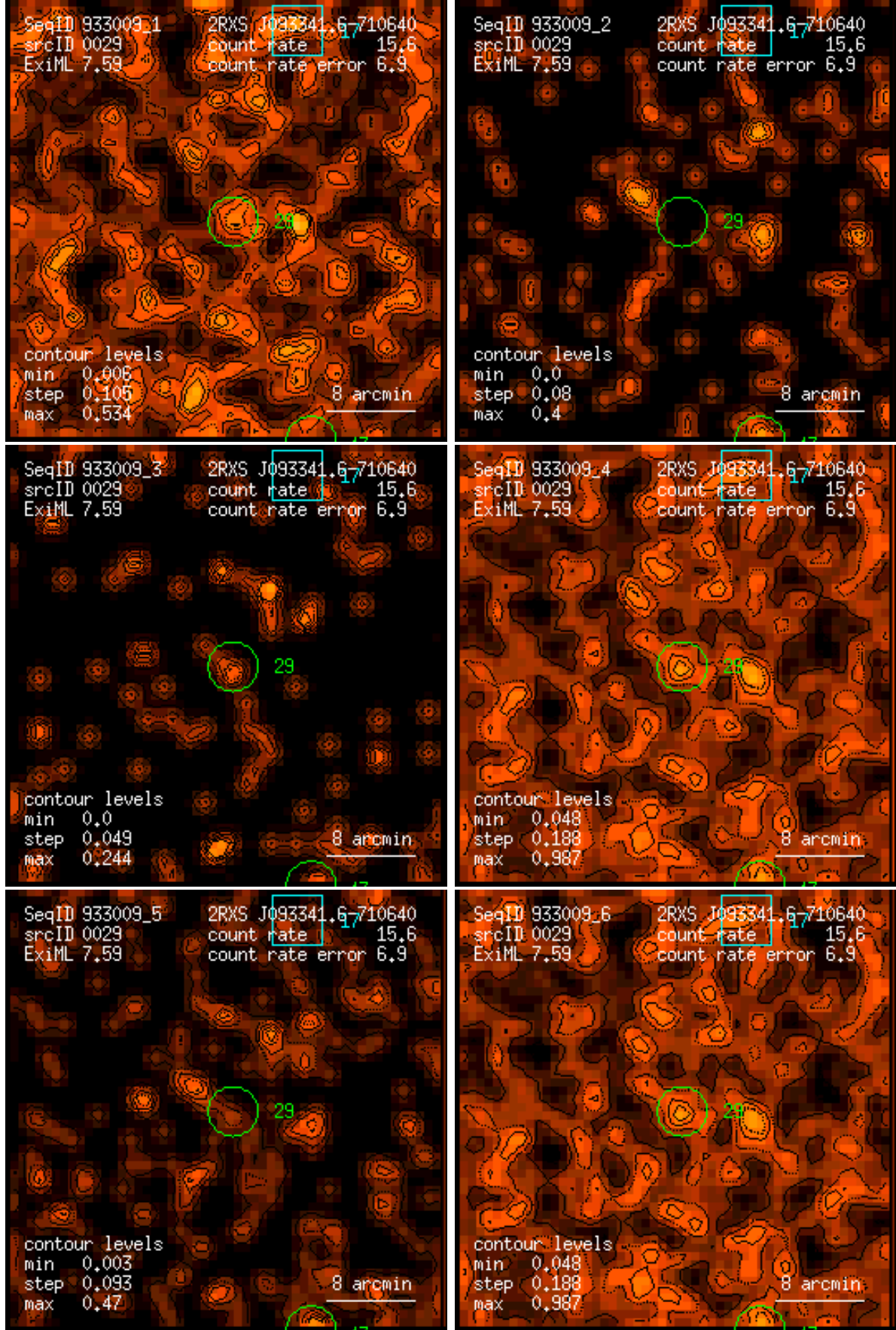
Figure 29: RASS 933009: detection 0029: band rate images, Gaussian filter: (1) PSPC channels 11 – 41, (2) 52 – 90, (3) 91 – 201, (4) 11 – 235, (5) 52 – 201, (6) 11 – 201. Broad band rates in counts/ks. Band rate contour levels in counts/ks/arcmin 2 .
