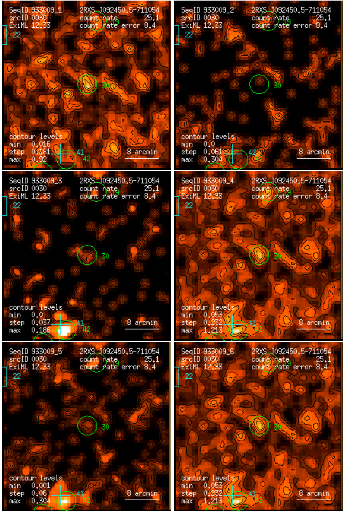
Figure 30: RASS 933009: detection 0030: band rate images, Gaussian filter: (1) PSPC channels 11 – 41, (2) 52 – 90, (3) 91 – 201, (4) 11 – 235, (5) 52 – 201, (6) 11 – 201. Broad band rates in counts/ks. Band rate contour levels in counts/ks/arcmin 2 .
