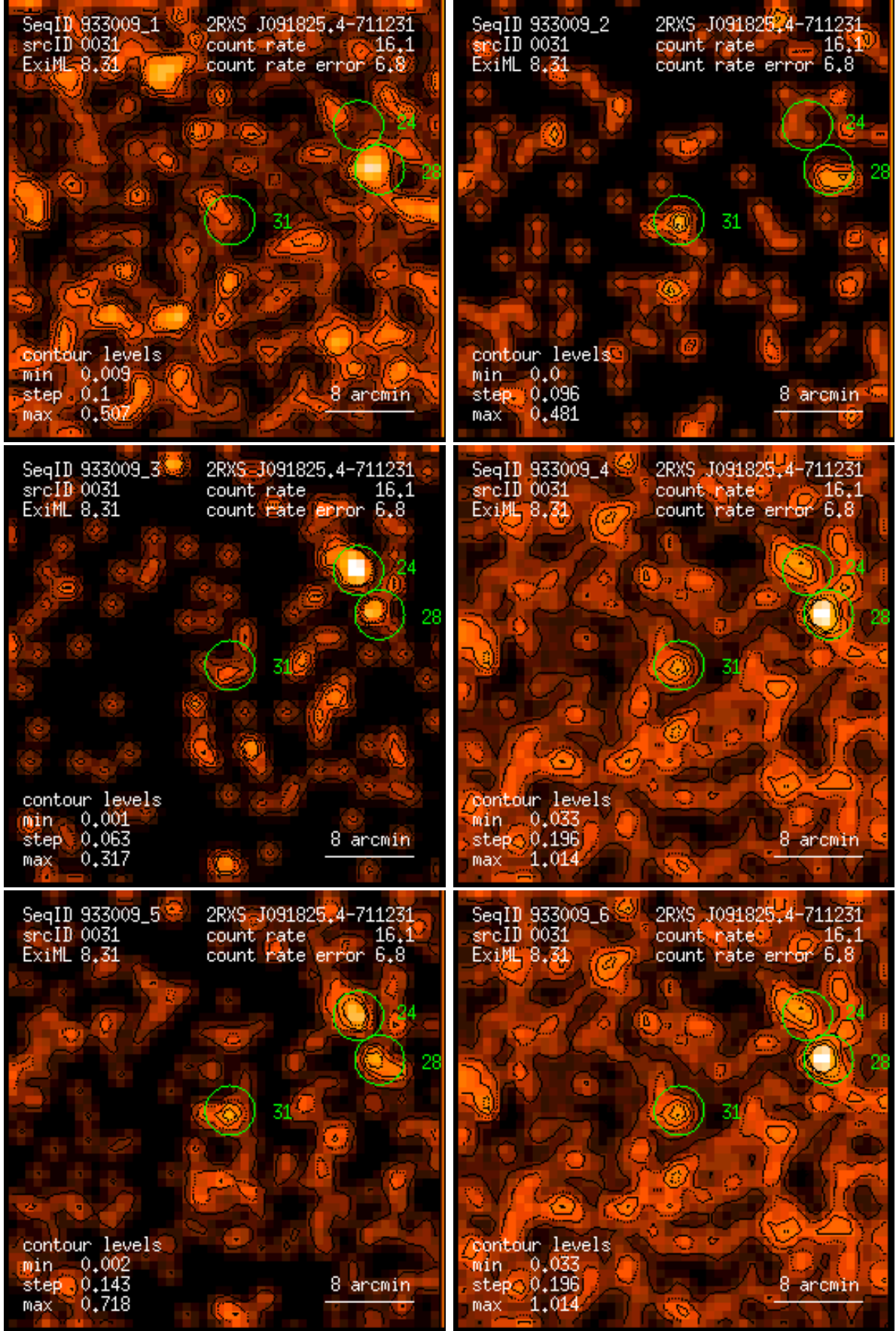
Figure 31: RASS 933009: detection 0031: band rate images, Gaussian filter: (1) PSPC channels 11 – 41, (2) 52 – 90, (3) 91 – 201, (4) 11 – 235, (5) 52 – 201, (6) 11 – 201. Broad band rates in counts/ks. Band rate contour levels in counts/ks/arcmin 2 .
