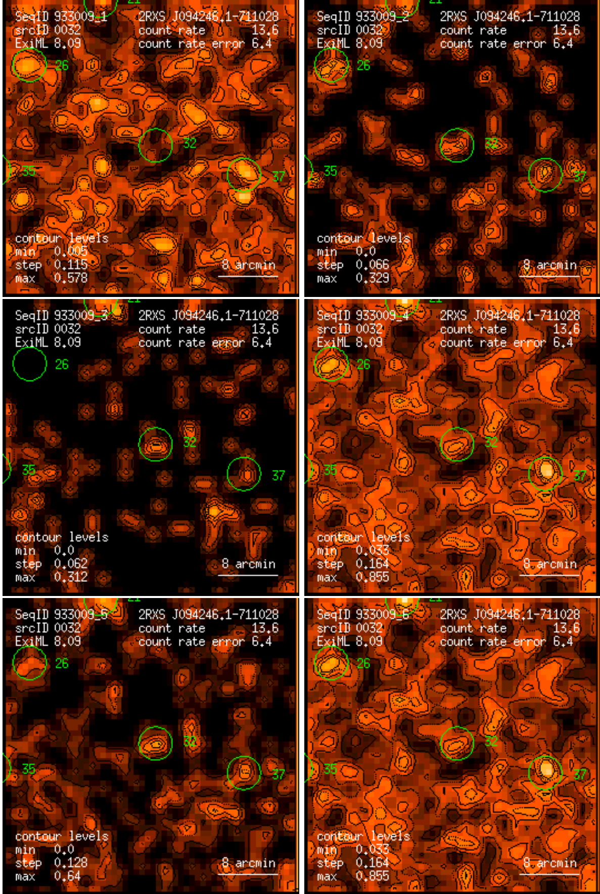
Figure 32: RASS 933009: detection 0032: band rate images, Gaussian filter: (1) PSPC channels 11 – 41, (2) 52 – 90, (3) 91 – 201, (4) 11 – 235, (5) 52 – 201, (6) 11 – 201. Broad band rates in counts/ks. Band rate contour levels in counts/ks/arcmin 2 .
