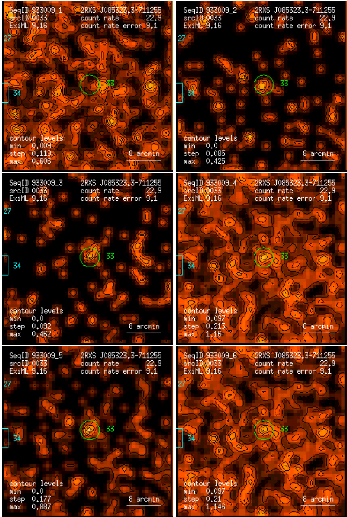
Figure 33: RASS 933009: detection 0033: band rate images, Gaussian filter: (1) PSPC channels 11 – 41, (2) 52 – 90, (3) 91 – 201, (4) 11 – 235, (5) 52 – 201, (6) 11 – 201. Broad band rates in counts/ks. Band rate contour levels in counts/ks/arcmin 2 .
