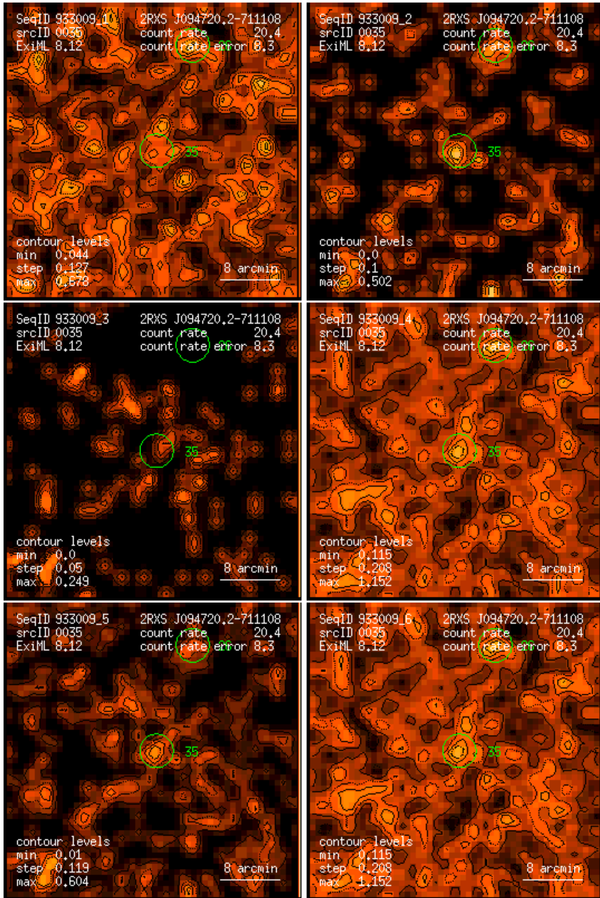
Figure 35: RASS 933009: detection 0035: band rate images, Gaussian filter: (1) PSPC channels 11 – 41, (2) 52 – 90, (3) 91 – 201, (4) 11 – 235, (5) 52 – 201, (6) 11 – 201. Broad band rates in counts/ks. Band rate contour levels in counts/ks/arcmin 2 .
