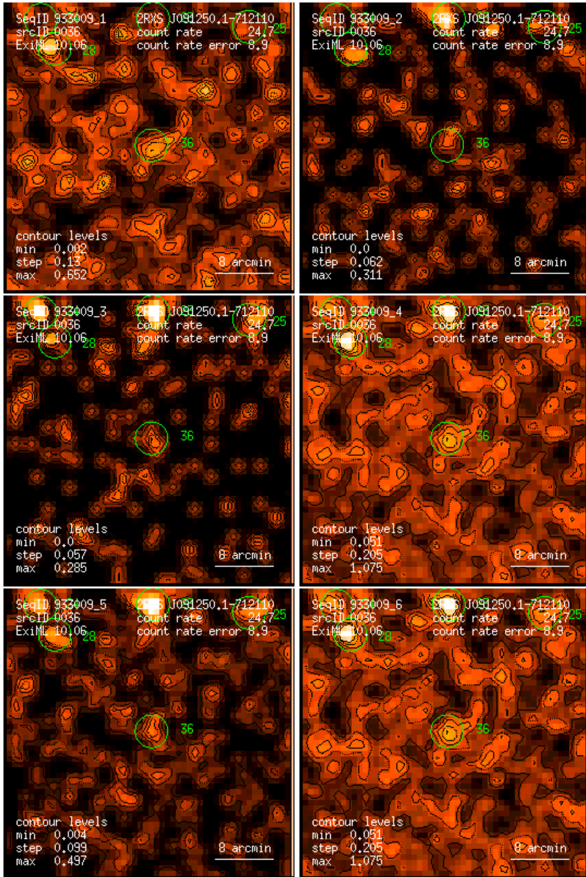
Figure 36: RASS 933009: detection 0036: band rate images, Gaussian filter: (1) PSPC channels 11 – 41, (2) 52 – 90, (3) 91 – 201, (4) 11 – 235, (5) 52 – 201, (6) 11 – 201. Broad band rates in counts/ks. Band rate contour levels in counts/ks/arcmin 2 .
