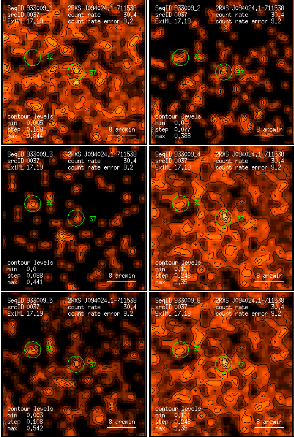
Figure 37: RASS 933009: detection 0037: band rate images, Gaussian filter: (1) PSPC channels 11 – 41, (2) 52 – 90, (3) 91 – 201, (4) 11 – 235, (5) 52 – 201, (6) 11 – 201. Broad band rates in counts/ks. Band rate contour levels in counts/ks/arcmin 2 .
