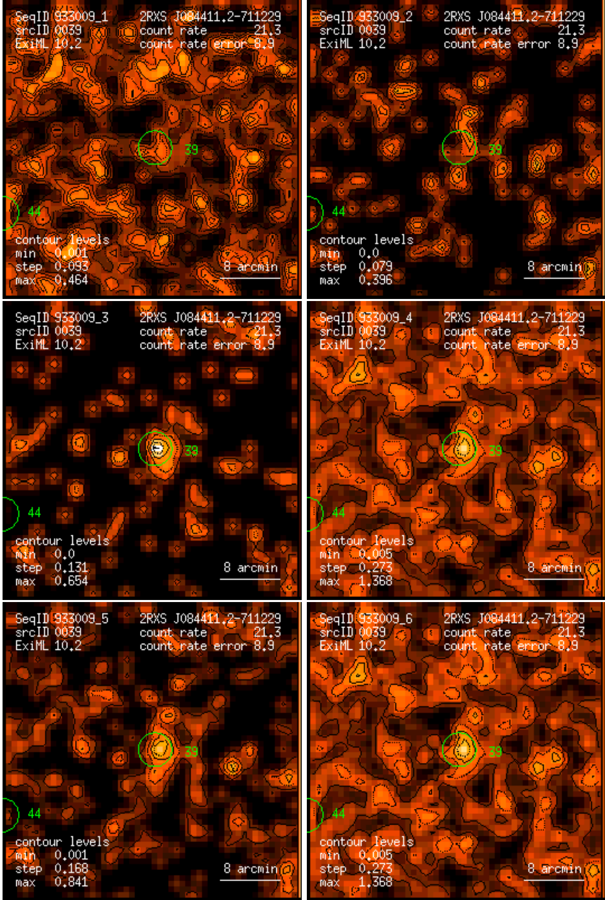
Figure 39: RASS 933009: detection 0039: band rate images, Gaussian filter: (1) PSPC channels 11 – 41, (2) 52 – 90, (3) 91 – 201, (4) 11 – 235, (5) 52 – 201, (6) 11 – 201. Broad band rates in counts/ks. Band rate contour levels in counts/ks/arcmin 2 .
