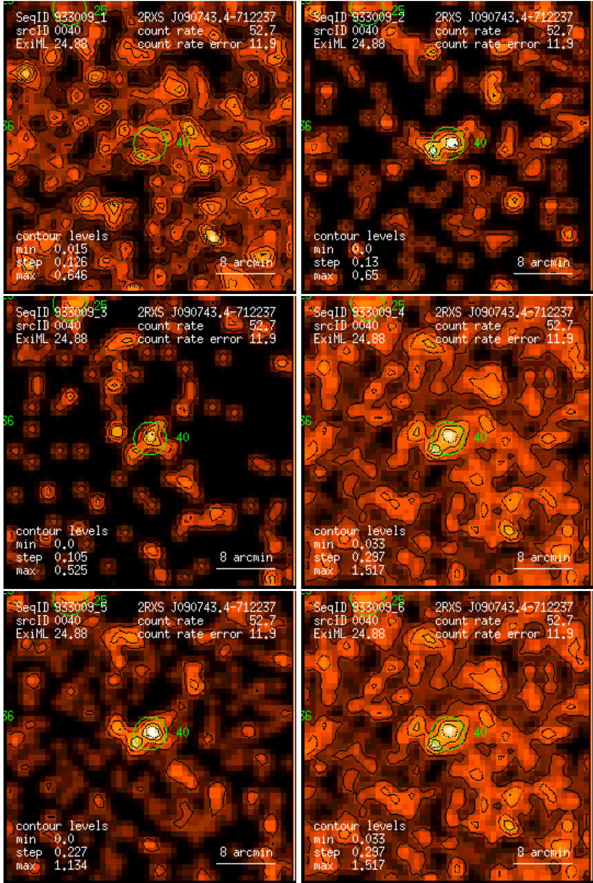
Figure 40: RASS 933009: detection 0040: band rate images, Gaussian filter: (1) PSPC channels 11 – 41, (2) 52 – 90, (3) 91 – 201, (4) 11 – 235, (5) 52 – 201, (6) 11 – 201. Broad band rates in counts/ks. Band rate contour levels in counts/ks/arcmin 2 .
