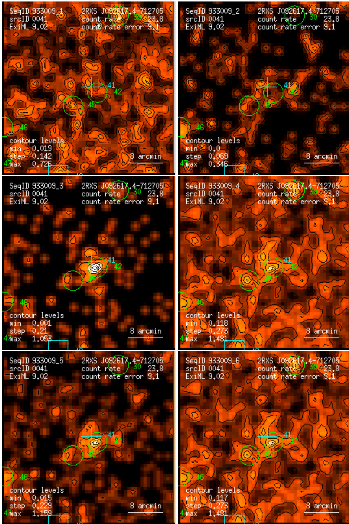
Figure 41: RASS 933009: detection 0041: band rate images, Gaussian filter: (1) PSPC channels 11 – 41, (2) 52 – 90, (3) 91 – 201, (4) 11 – 235, (5) 52 – 201, (6) 11 – 201. Broad band rates in counts/ks. Band rate contour levels in counts/ks/arcmin 2 .
