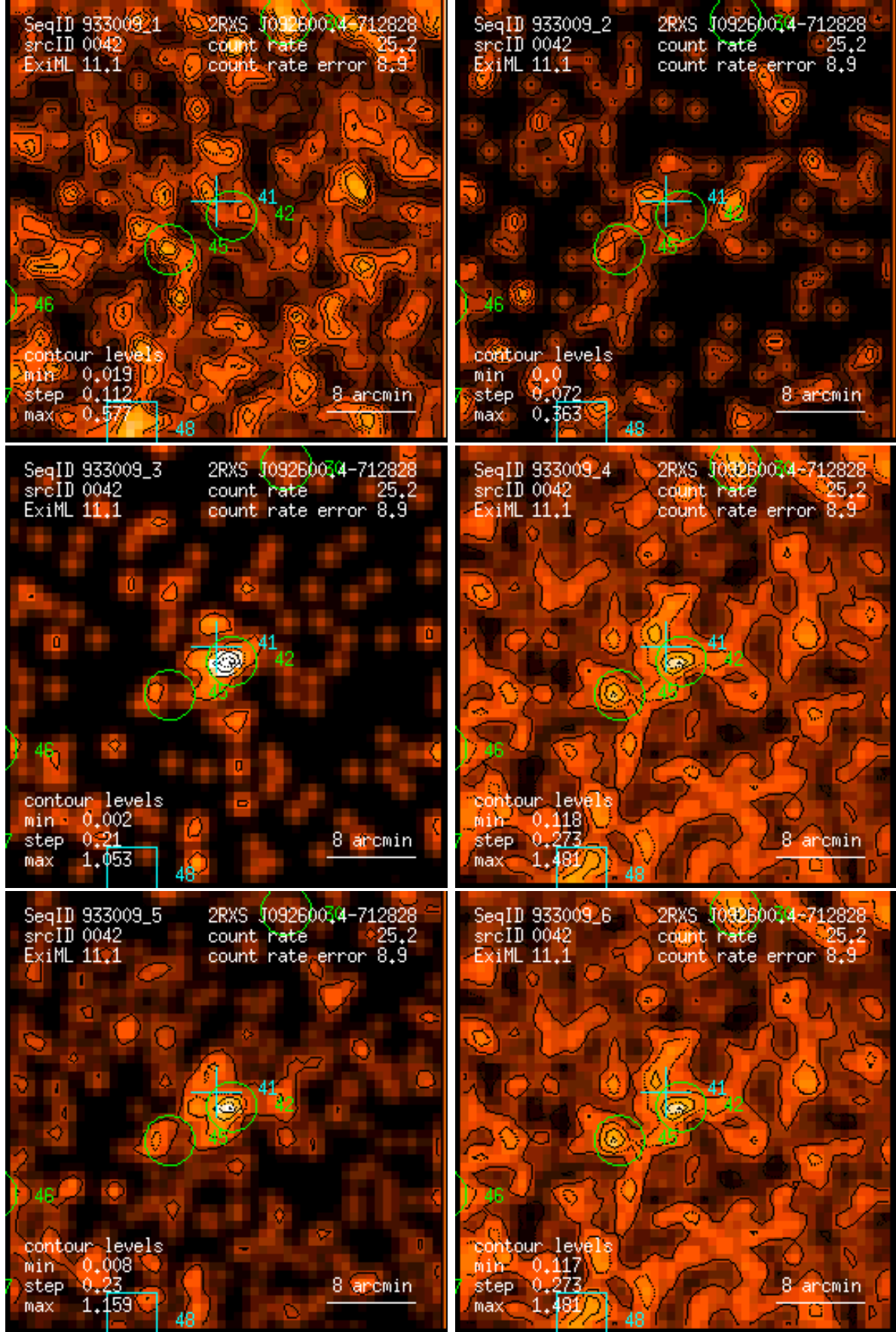
Figure 42: RASS 933009: detection 0042: band rate images, Gaussian filter: (1) PSPC channels 11 – 41, (2) 52 – 90, (3) 91 – 201, (4) 11 – 235, (5) 52 – 201, (6) 11 – 201. Broad band rates in counts/ks. Band rate contour levels in counts/ks/arcmin 2 .
