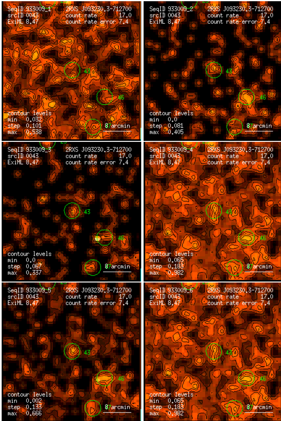
Figure 43: RASS 933009: detection 0043: band rate images, Gaussian filter: (1) PSPC channels 11 – 41, (2) 52 – 90, (3) 91 – 201, (4) 11 – 235, (5) 52 – 201, (6) 11 – 201. Broad band rates in counts/ks. Band rate contour levels in counts/ks/arcmin 2 .
