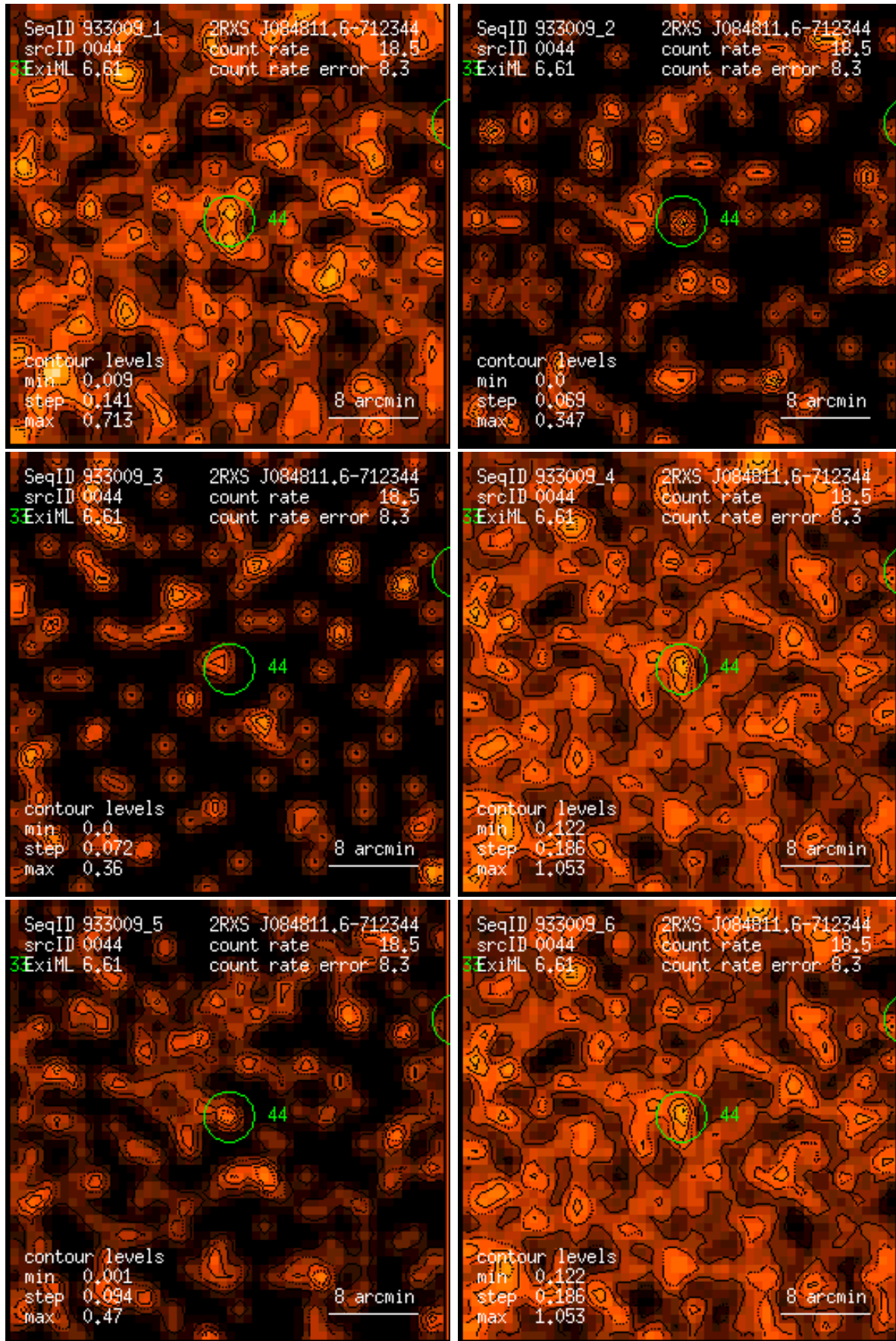
Figure 44: RASS 933009: detection 0044: band rate images, Gaussian filter: (1) PSPC channels 11 – 41, (2) 52 – 90, (3) 91 – 201, (4) 11 – 235, (5) 52 – 201, (6) 11 – 201. Broad band rates in counts/ks. Band rate contour levels in counts/ks/arcmin 2 .
