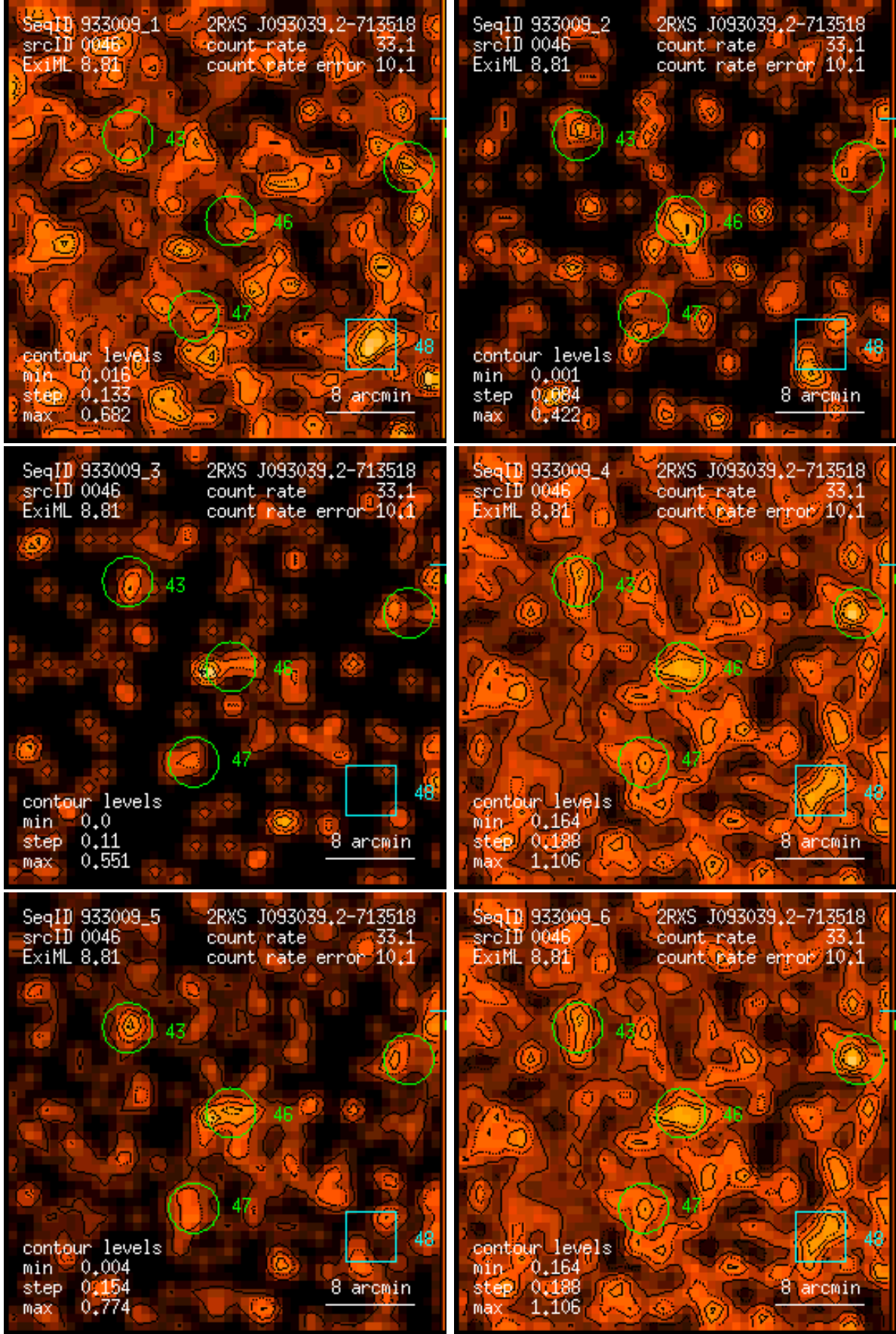
Figure 46: RASS 933009: detection 0046: band rate images, Gaussian filter: (1) PSPC channels 11 – 41, (2) 52 – 90, (3) 91 – 201, (4) 11 – 235, (5) 52 – 201, (6) 11 – 201. Broad band rates in counts/ks. Band rate contour levels in counts/ks/arcmin 2 .
