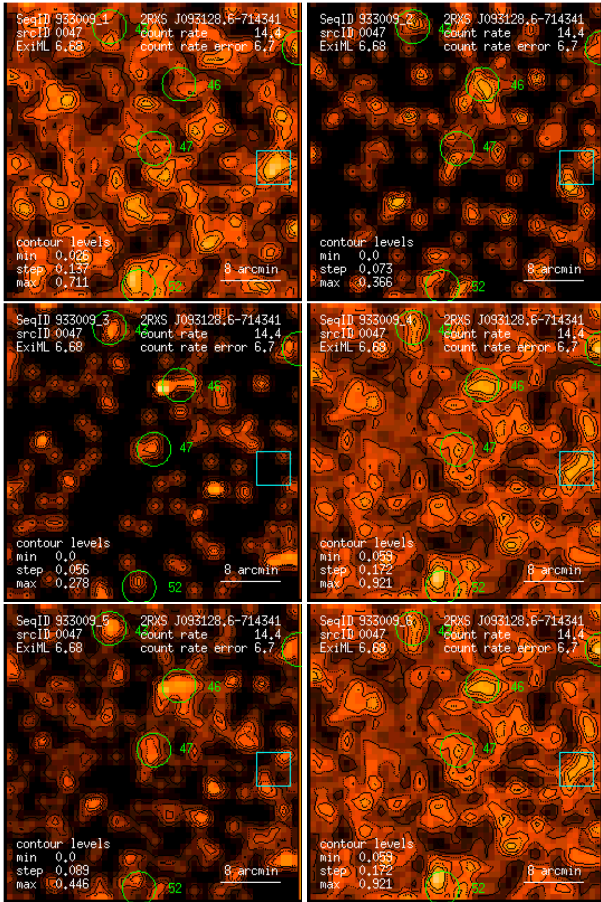
Figure 47: RASS 933009: detection 0047: band rate images, Gaussian filter: (1) PSPC channels 11 – 41, (2) 52 – 90, (3) 91 – 201, (4) 11 – 235, (5) 52 – 201, (6) 11 – 201. Broad band rates in counts/ks. Band rate contour levels in counts/ks/arcmin 2 .
