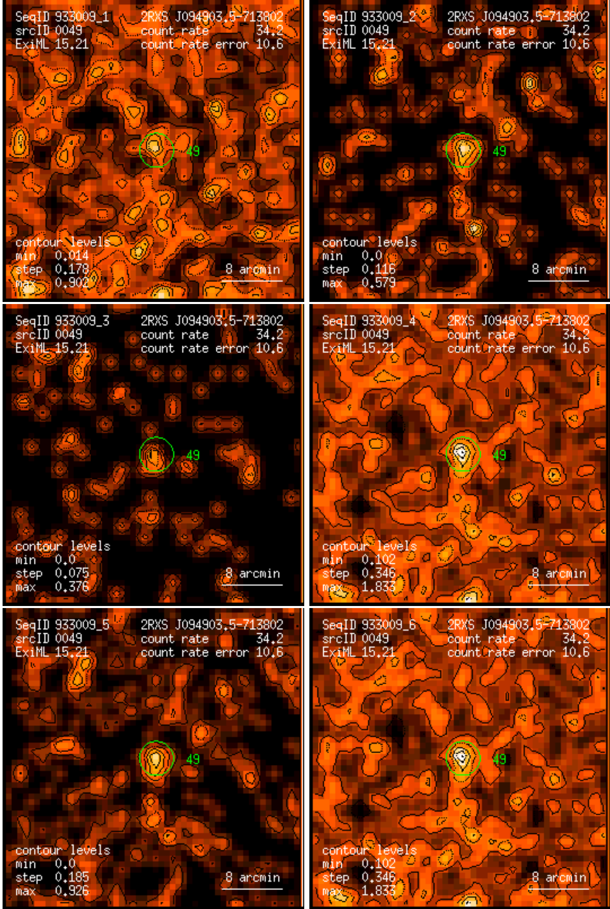
Figure 49: RASS 933009: detection 0049: band rate images, Gaussian filter: (1) PSPC channels 11 – 41, (2) 52 – 90, (3) 91 – 201, (4) 11 – 235, (5) 52 – 201, (6) 11 – 201. Broad band rates in counts/ks. Band rate contour levels in counts/ks/arcmin 2 .
