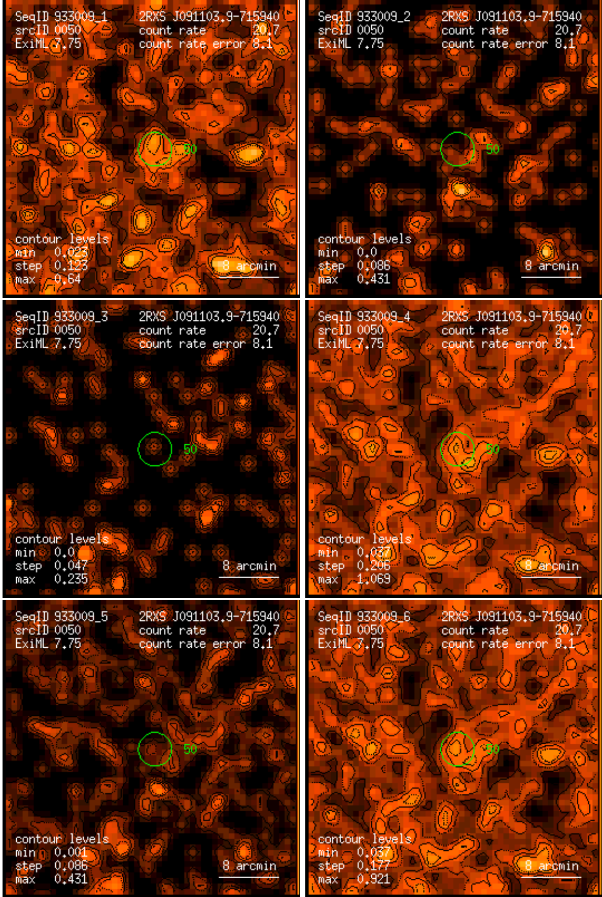
Figure 50: RASS 933009: detection 0050: band rate images, Gaussian filter: (1) PSPC channels 11 – 41, (2) 52 – 90, (3) 91 – 201, (4) 11 – 235, (5) 52 – 201, (6) 11 – 201. Broad band rates in counts/ks. Band rate contour levels in counts/ks/arcmin 2 .
