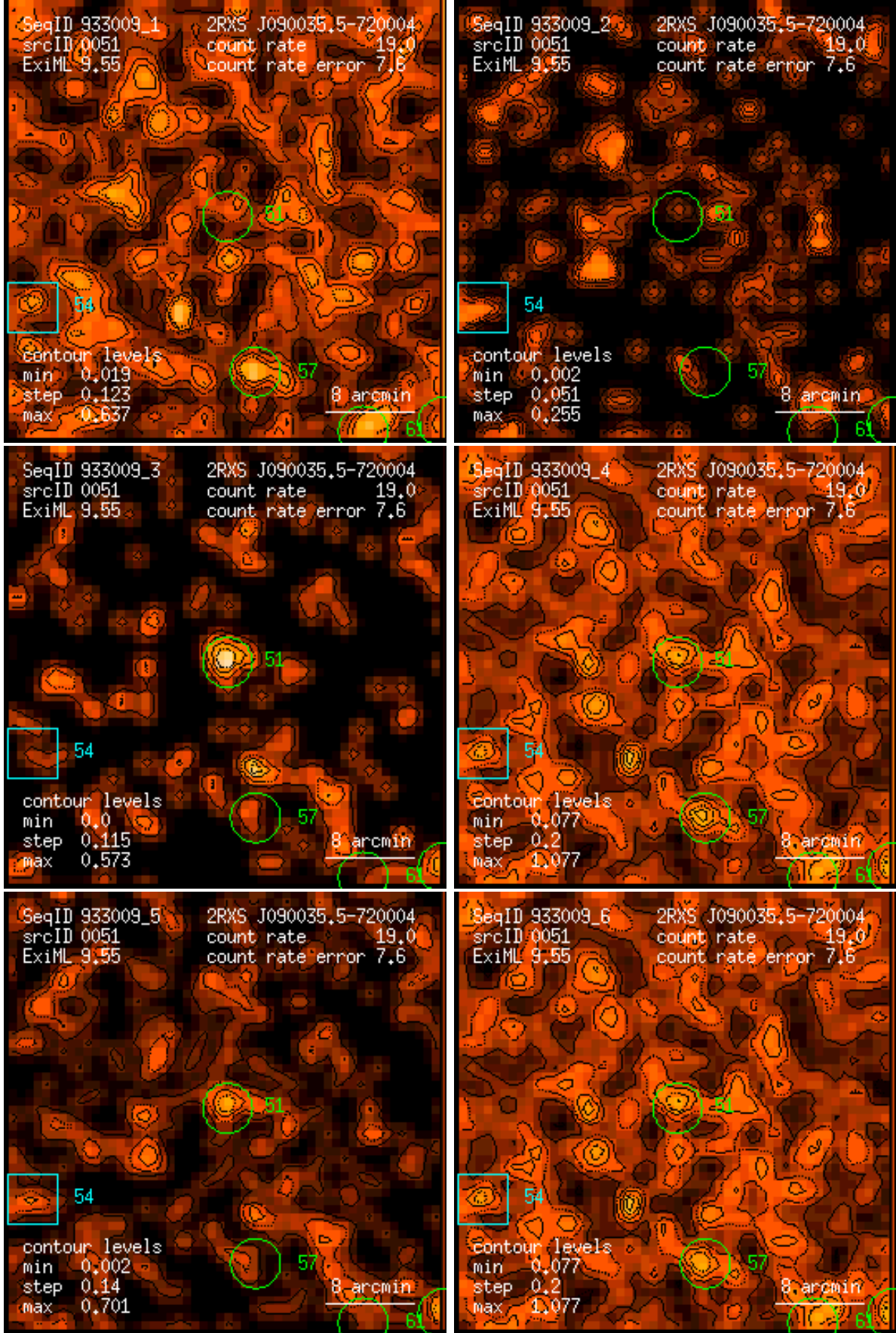
Figure 51: RASS 933009: detection 0051: band rate images, Gaussian filter: (1) PSPC channels 11 – 41, (2) 52 – 90, (3) 91 – 201, (4) 11 – 235, (5) 52 – 201, (6) 11 – 201. Broad band rates in counts/ks. Band rate contour levels in counts/ks/arcmin 2 .
