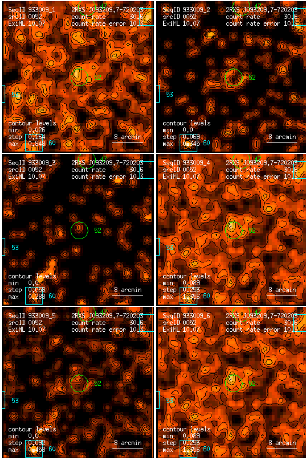
Figure 52: RASS 933009: detection 0052: band rate images, Gaussian filter: (1) PSPC channels 11 – 41, (2) 52 – 90, (3) 91 – 201, (4) 11 – 235, (5) 52 – 201, (6) 11 – 201. Broad band rates in counts/ks. Band rate contour levels in counts/ks/arcmin 2 .
