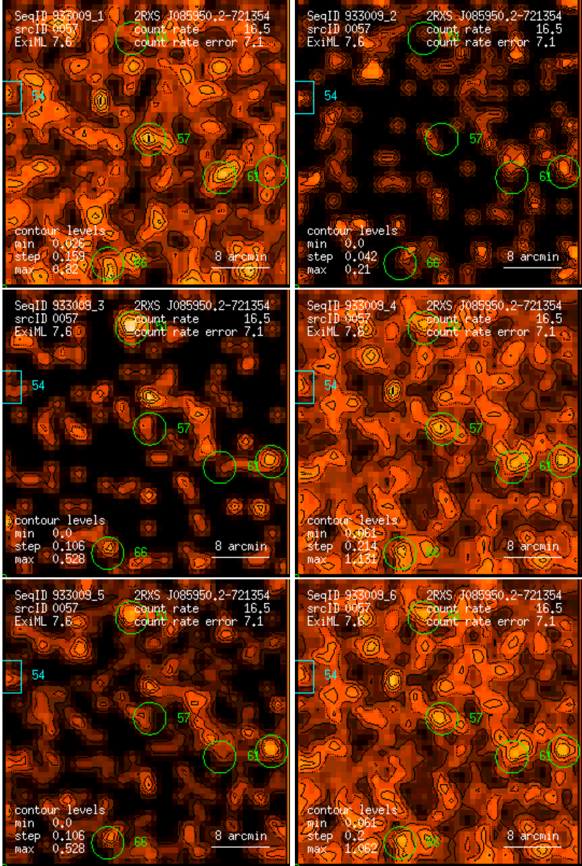
Figure 57: RASS 933009: detection 0057: band rate images, Gaussian filter: (1) PSPC channels 11 – 41, (2) 52 – 90, (3) 91 – 201, (4) 11 – 235, (5) 52 – 201, (6) 11 – 201. Broad band rates in counts/ks. Band rate contour levels in counts/ks/arcmin 2 .
