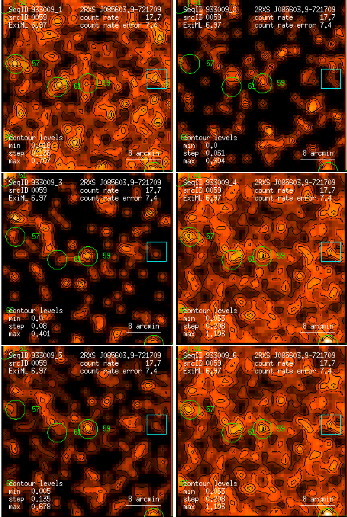
Figure 59: RASS 933009: detection 0059: band rate images, Gaussian filter: (1) PSPC channels 11 – 41, (2) 52 – 90, (3) 91 – 201, (4) 11 – 235, (5) 52 – 201, (6) 11 – 201. Broad band rates in counts/ks. Band rate contour levels in counts/ks/arcmin 2 .
