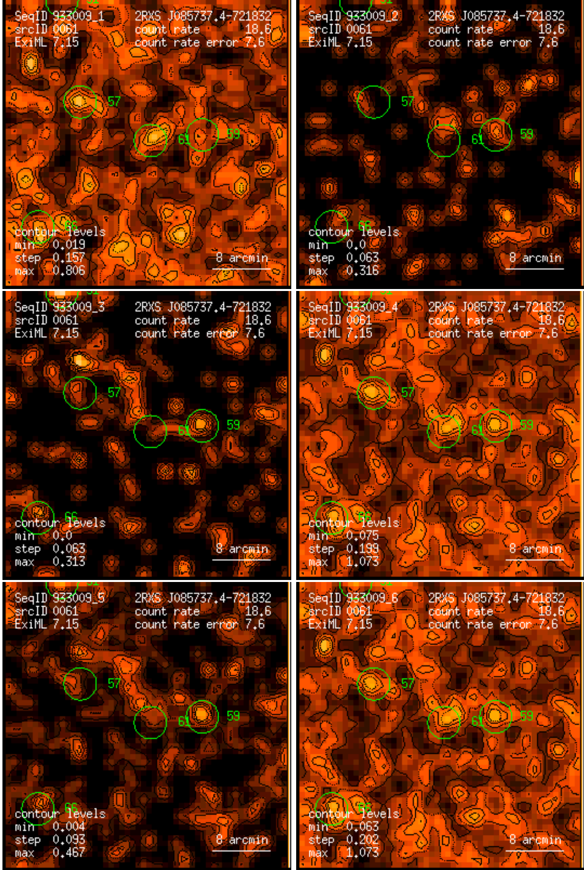
Figure 61: RASS 933009: detection 0061: band rate images, Gaussian filter: (1) PSPC channels 11 – 41, (2) 52 – 90, (3) 91 – 201, (4) 11 – 235, (5) 52 – 201, (6) 11 – 201. Broad band rates in counts/ks. Band rate contour levels in counts/ks/arcmin 2 .
