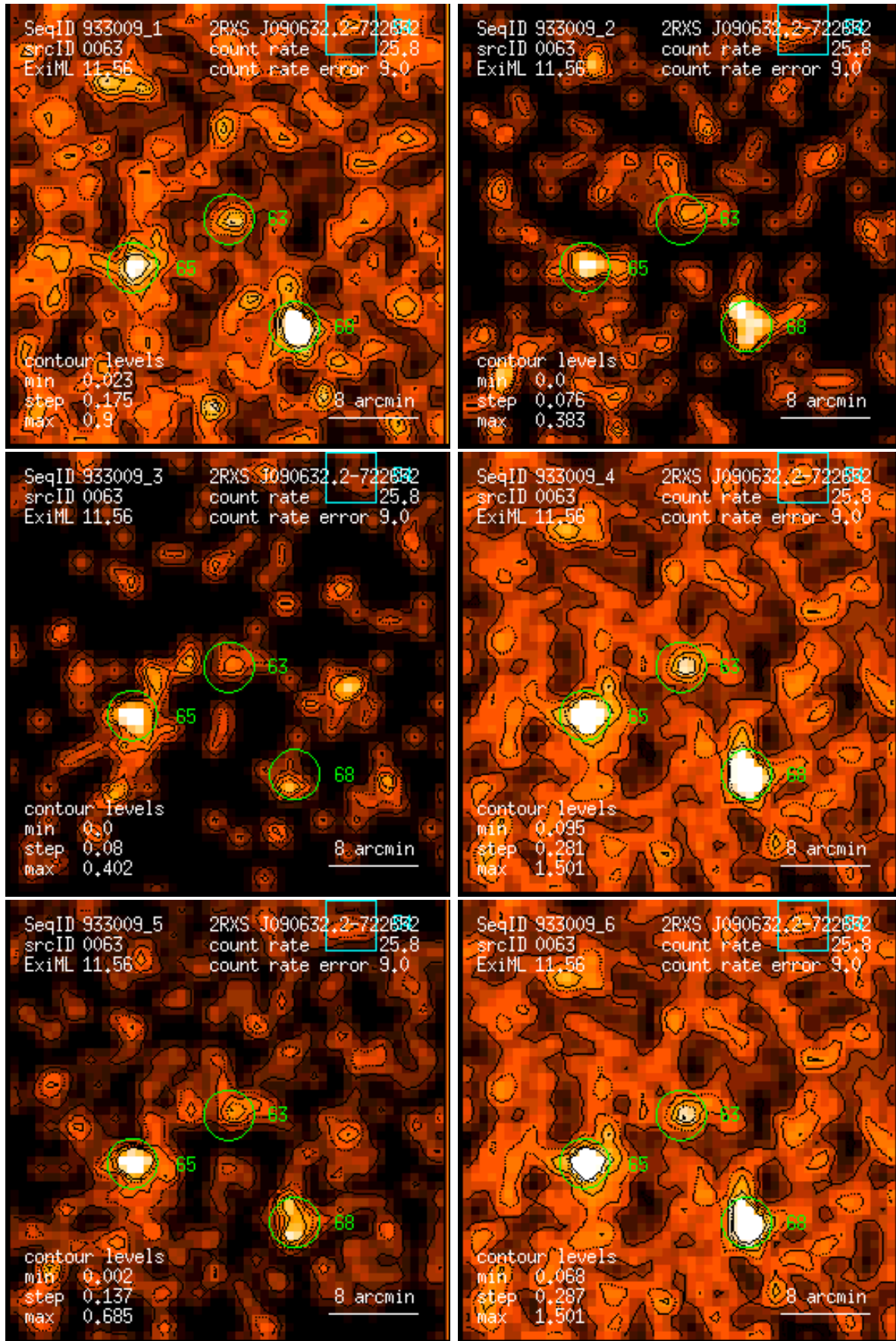
Figure 63: RASS 933009: detection 0063: band rate images, Gaussian filter: (1) PSPC channels 11 – 41, (2) 52 – 90, (3) 91 – 201, (4) 11 – 235, (5) 52 – 201, (6) 11 – 201. Broad band rates in counts/ks. Band rate contour levels in counts/ks/arcmin 2 .
