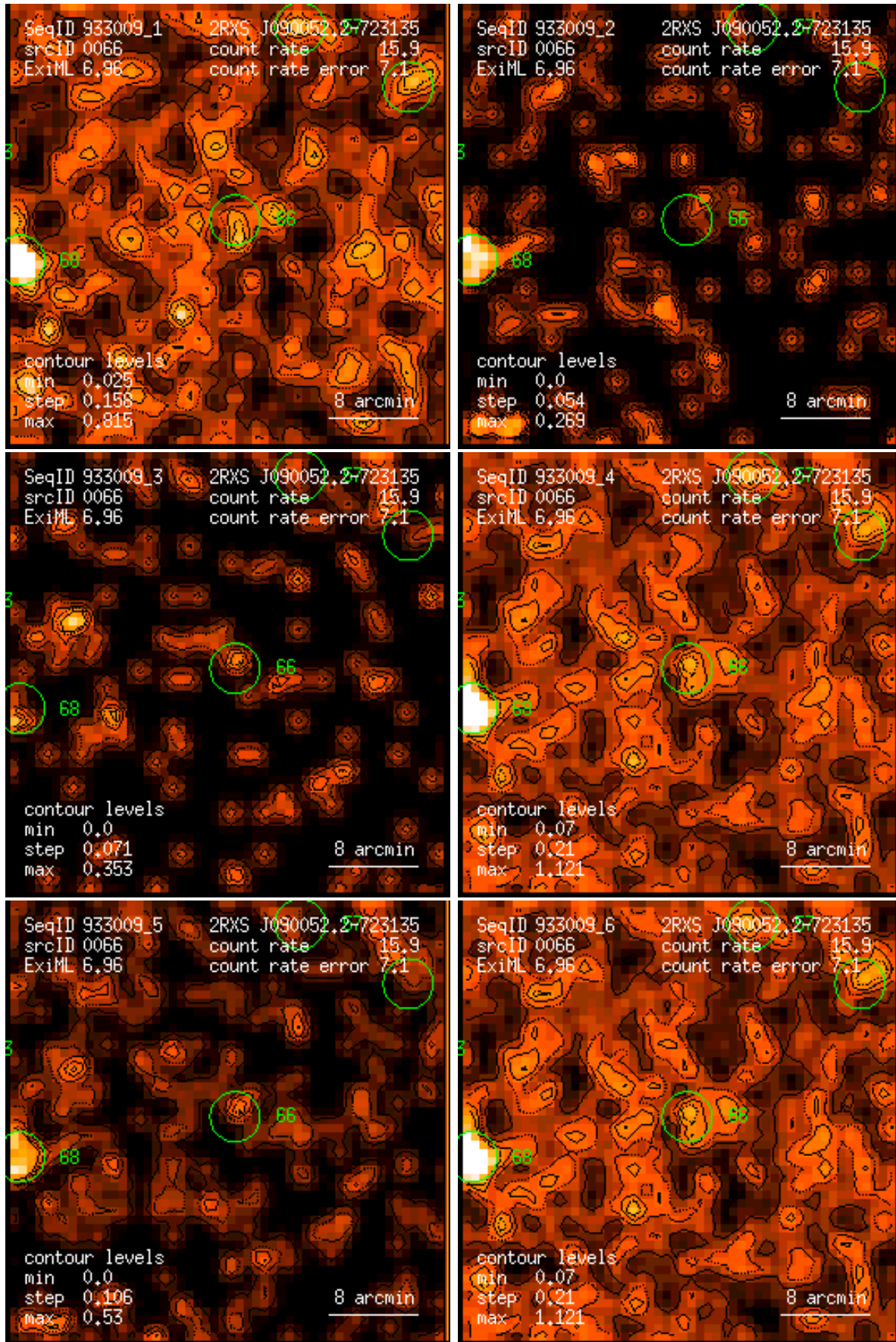
Figure 66: RASS 933009: detection 0066: band rate images, Gaussian filter: (1) PSPC channels 11 – 41, (2) 52 – 90, (3) 91 – 201, (4) 11 – 235, (5) 52 – 201, (6) 11 – 201. Broad band rates in counts/ks. Band rate contour levels in counts/ks/arcmin 2 .
