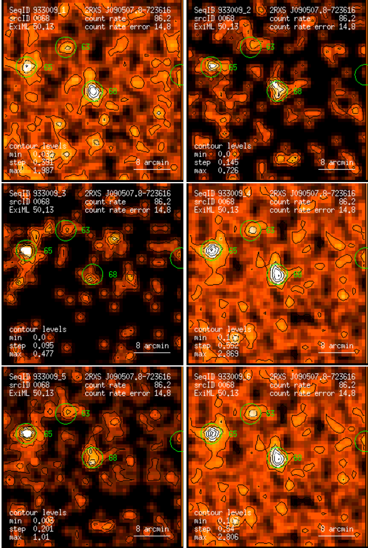
Figure 68: RASS 933009: detection 0068: band rate images, Gaussian filter: (1) PSPC channels 11 – 41, (2) 52 – 90, (3) 91 – 201, (4) 11 – 235, (5) 52 – 201, (6) 11 – 201. Broad band rates in counts/ks. Band rate contour levels in counts/ks/arcmin 2 .
