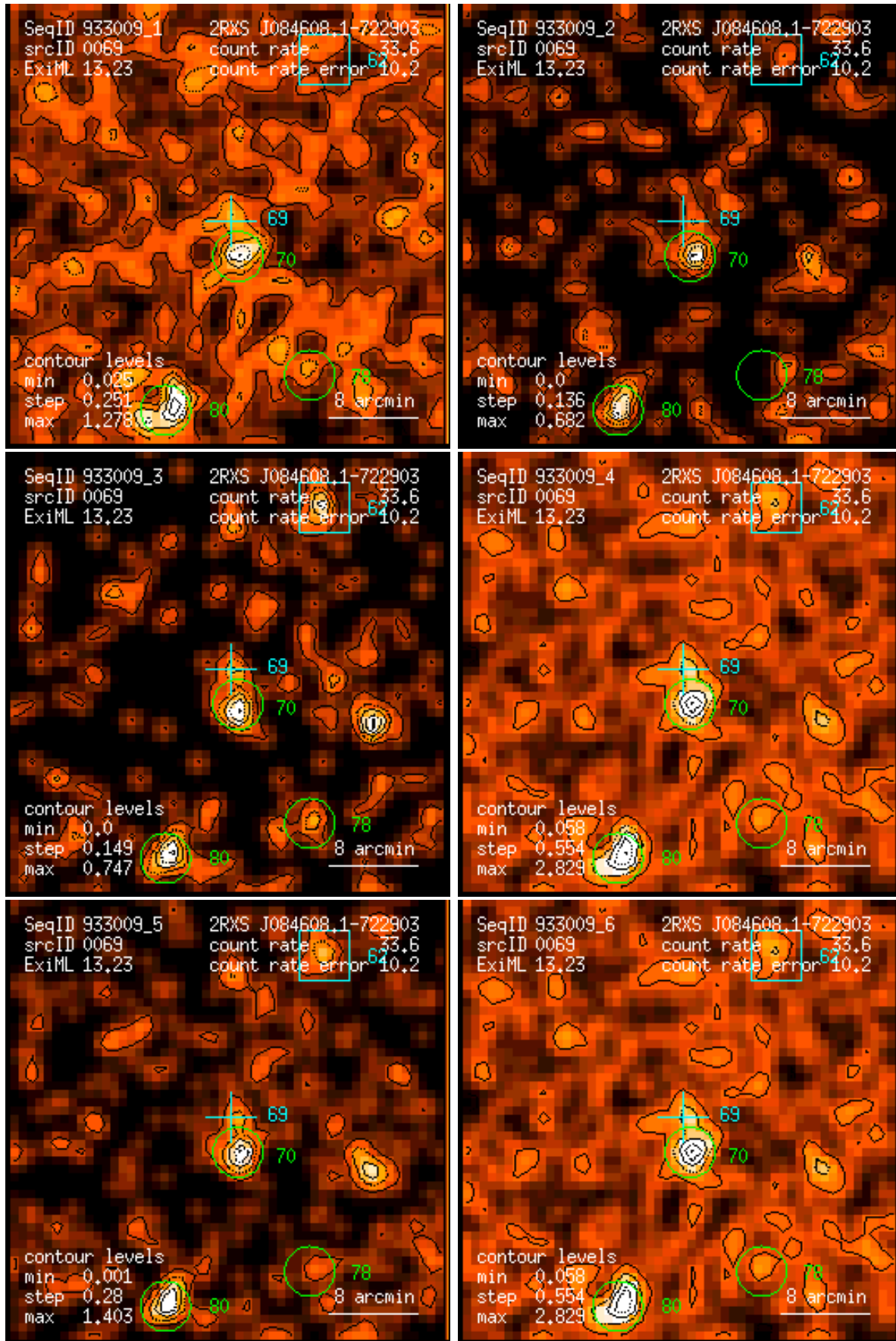
Figure 69: RASS 933009: detection 0069: band rate images, Gaussian filter: (1) PSPC channels 11 – 41, (2) 52 – 90, (3) 91 – 201, (4) 11 – 235, (5) 52 – 201, (6) 11 – 201. Broad band rates in counts/ks. Band rate contour levels in counts/ks/arcmin 2 .
