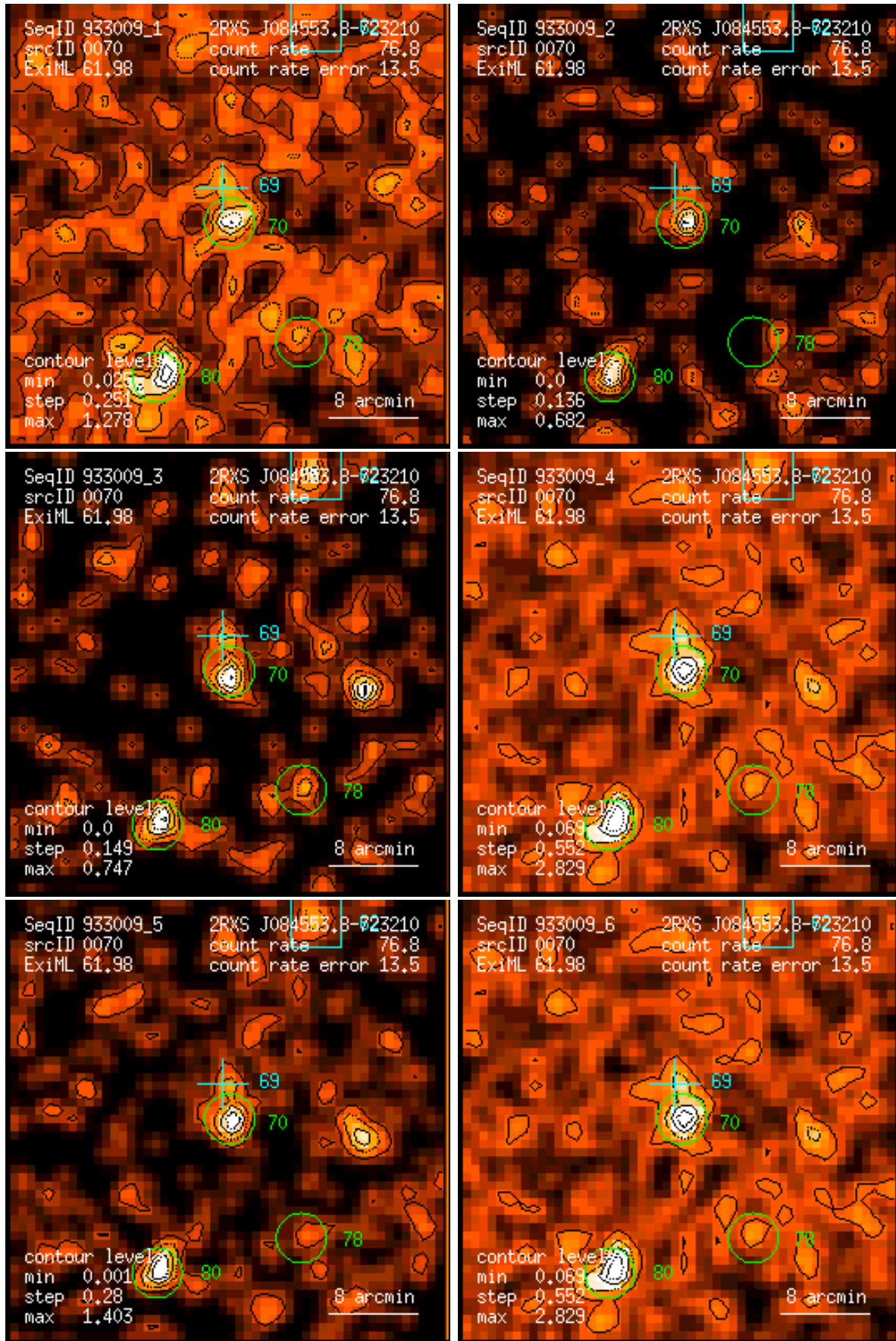
Figure 70: RASS 933009: detection 0070: band rate images, Gaussian filter: (1) PSPC channels 11 – 41, (2) 52 – 90, (3) 91 – 201, (4) 11 – 235, (5) 52 – 201, (6) 11 – 201. Broad band rates in counts/ks. Band rate contour levels in counts/ks/arcmin 2 .
