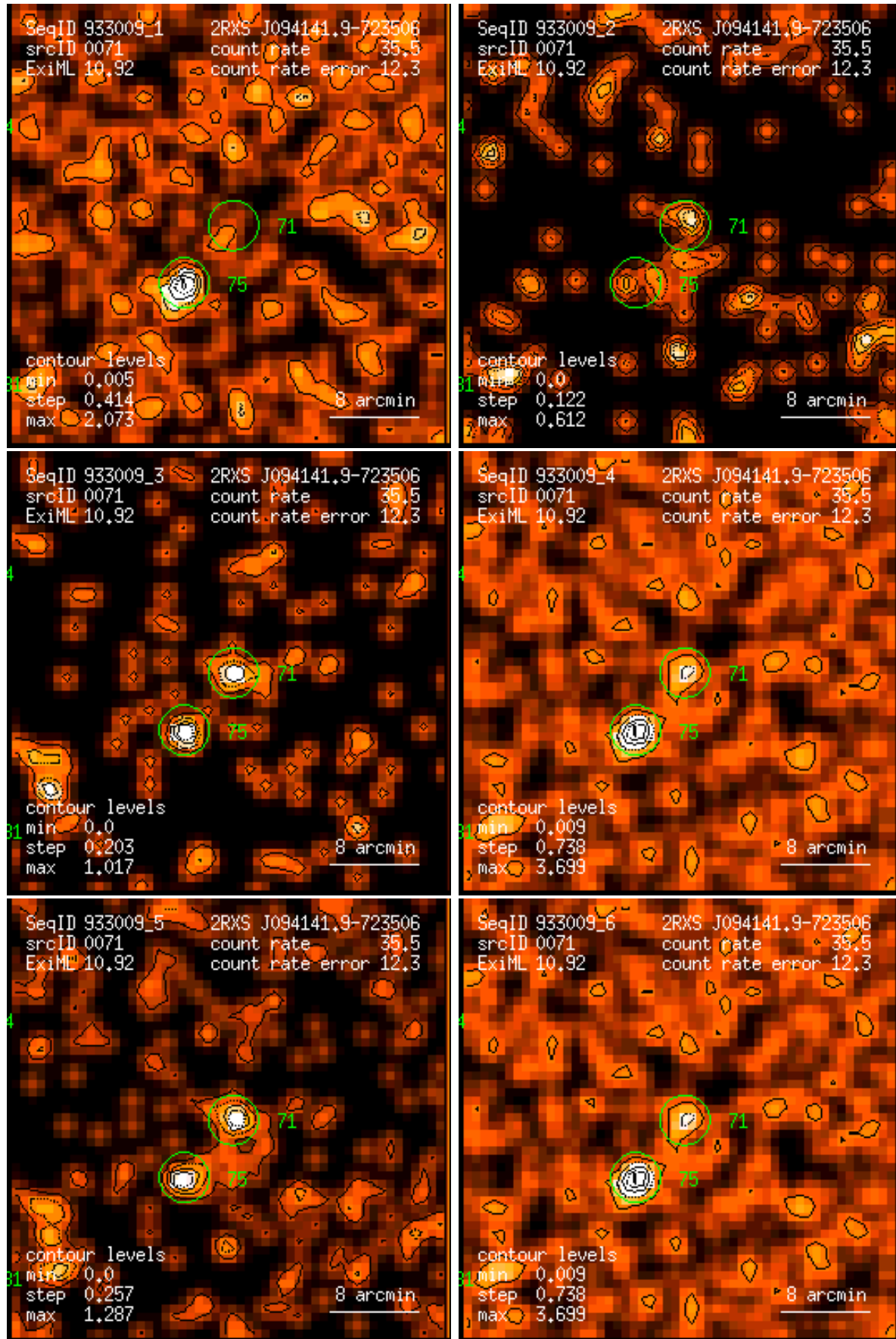
Figure 71: RASS 933009: detection 0071: band rate images, Gaussian filter: (1) PSPC channels 11 – 41, (2) 52 – 90, (3) 91 – 201, (4) 11 – 235, (5) 52 – 201, (6) 11 – 201. Broad band rates in counts/ks. Band rate contour levels in counts/ks/arcmin 2 .
