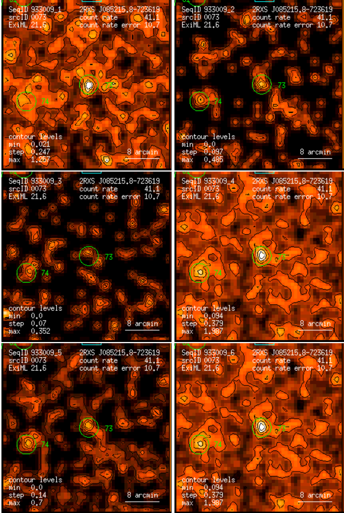
Figure 73: RASS 933009: detection 0073: band rate images, Gaussian filter: (1) PSPC channels 11 – 41, (2) 52 – 90, (3) 91 – 201, (4) 11 – 235, (5) 52 – 201, (6) 11 – 201. Broad band rates in counts/ks. Band rate contour levels in counts/ks/arcmin 2 .
