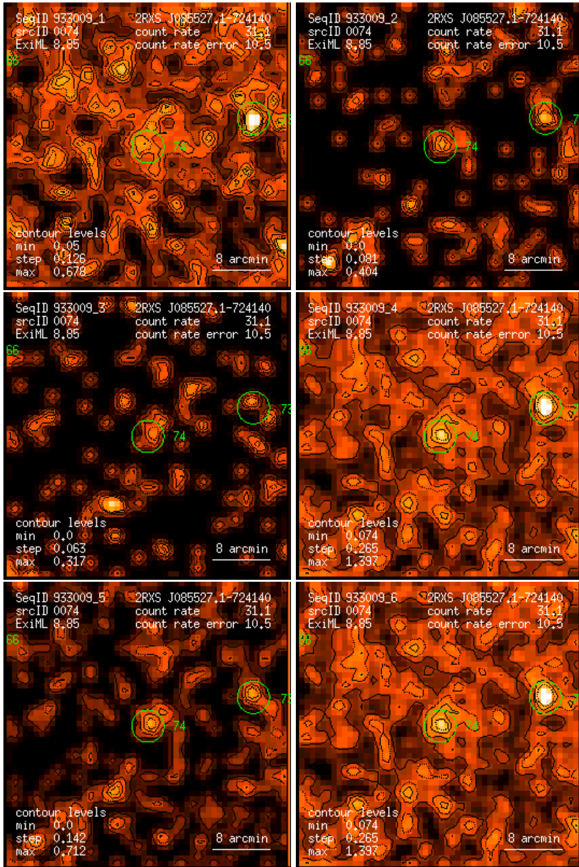
Figure 74: RASS 933009: detection 0074: band rate images, Gaussian filter: (1) PSPC channels 11 – 41, (2) 52 – 90, (3) 91 – 201, (4) 11 – 235, (5) 52 – 201, (6) 11 – 201. Broad band rates in counts/ks. Band rate contour levels in counts/ks/arcmin 2 .
