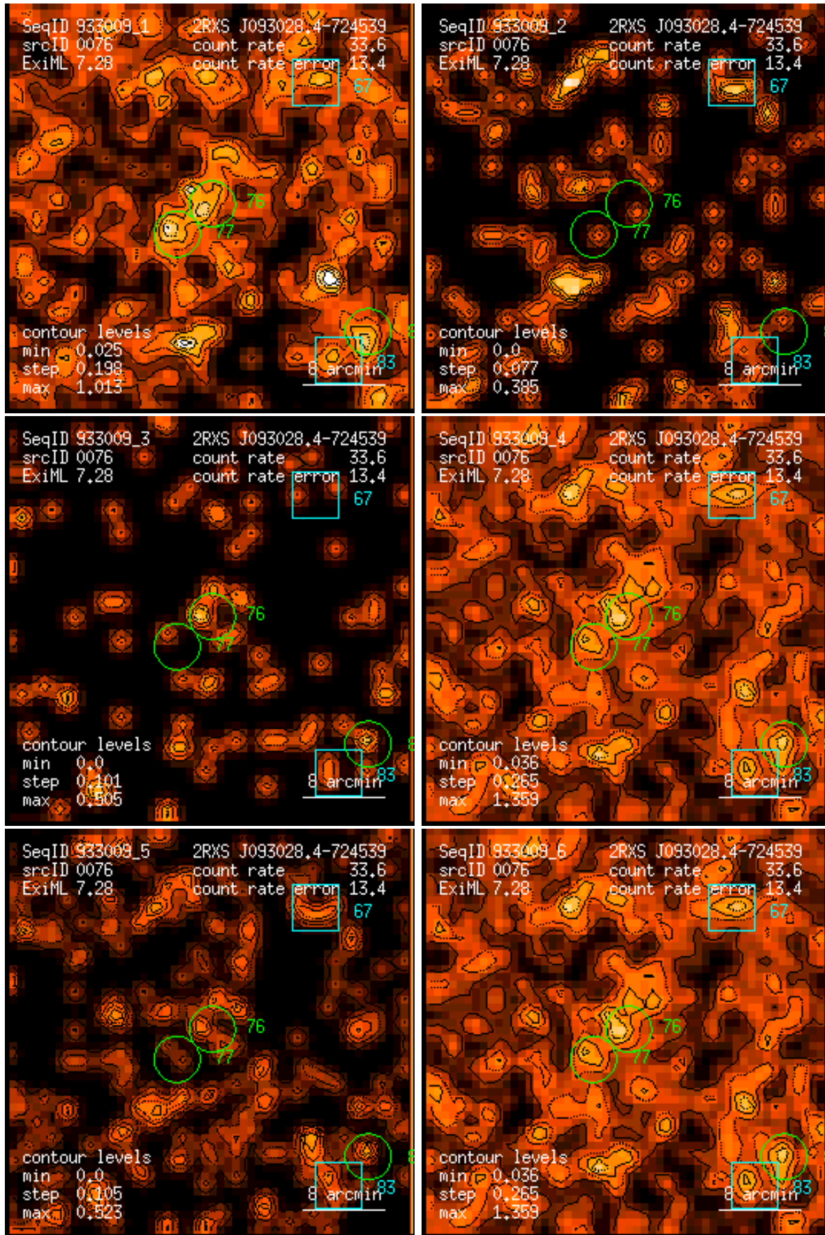
Figure 76: RASS 933009: detection 0076: band rate images, Gaussian filter: (1) PSPC channels 11 – 41, (2) 52 – 90, (3) 91 – 201, (4) 11 – 235, (5) 52 – 201, (6) 11 – 201. Broad band rates in counts/ks. Band rate contour levels in counts/ks/arcmin 2 .
