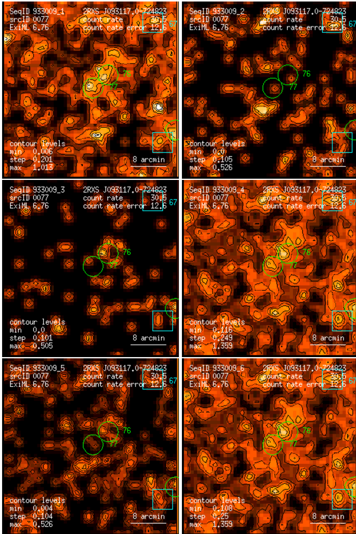
Figure 77: RASS 933009: detection 0077: band rate images, Gaussian filter: (1) PSPC channels 11 – 41, (2) 52 – 90, (3) 91 – 201, (4) 11 – 235, (5) 52 – 201, (6) 11 – 201. Broad band rates in counts/ks. Band rate contour levels in counts/ks/arcmin 2 .
