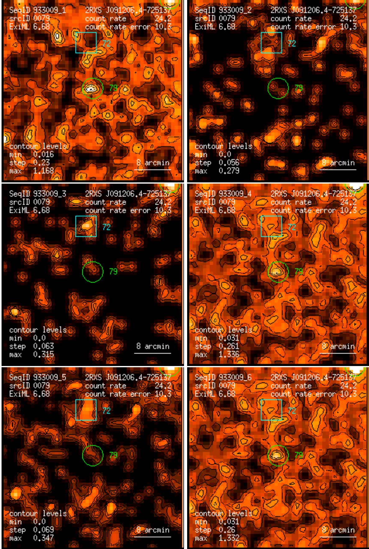
Figure 79: RASS 933009: detection 0079: band rate images, Gaussian filter: (1) PSPC channels 11 – 41, (2) 52 – 90, (3) 91 – 201, (4) 11 – 235, (5) 52 – 201, (6) 11 – 201. Broad band rates in counts/ks. Band rate contour levels in counts/ks/arcmin 2 .
