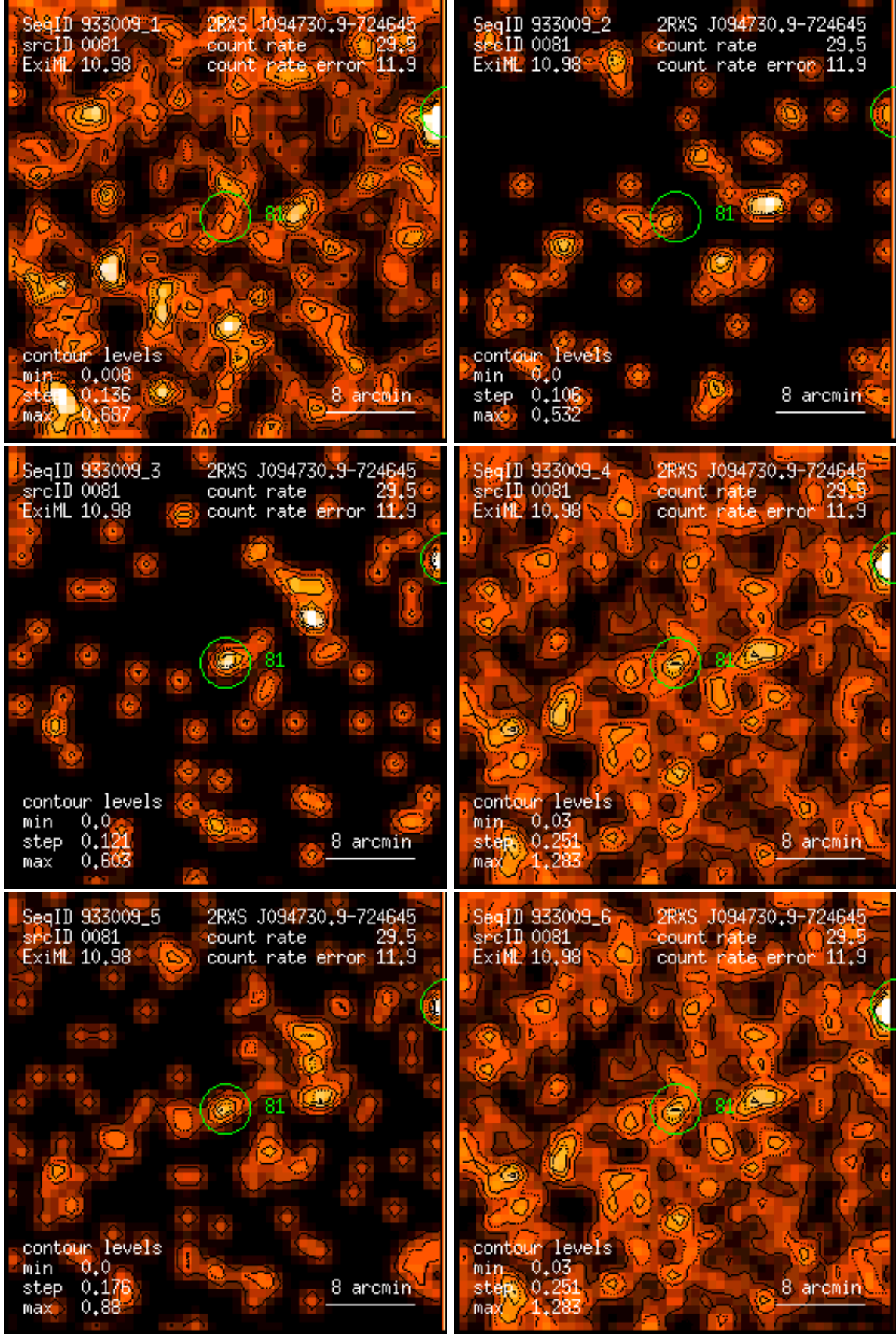
Figure 81: RASS 933009: detection 0081: band rate images, Gaussian filter: (1) PSPC channels 11 – 41, (2) 52 – 90, (3) 91 – 201, (4) 11 – 235, (5) 52 – 201, (6) 11 – 201. Broad band rates in counts/ks. Band rate contour levels in counts/ks/arcmin 2 .
