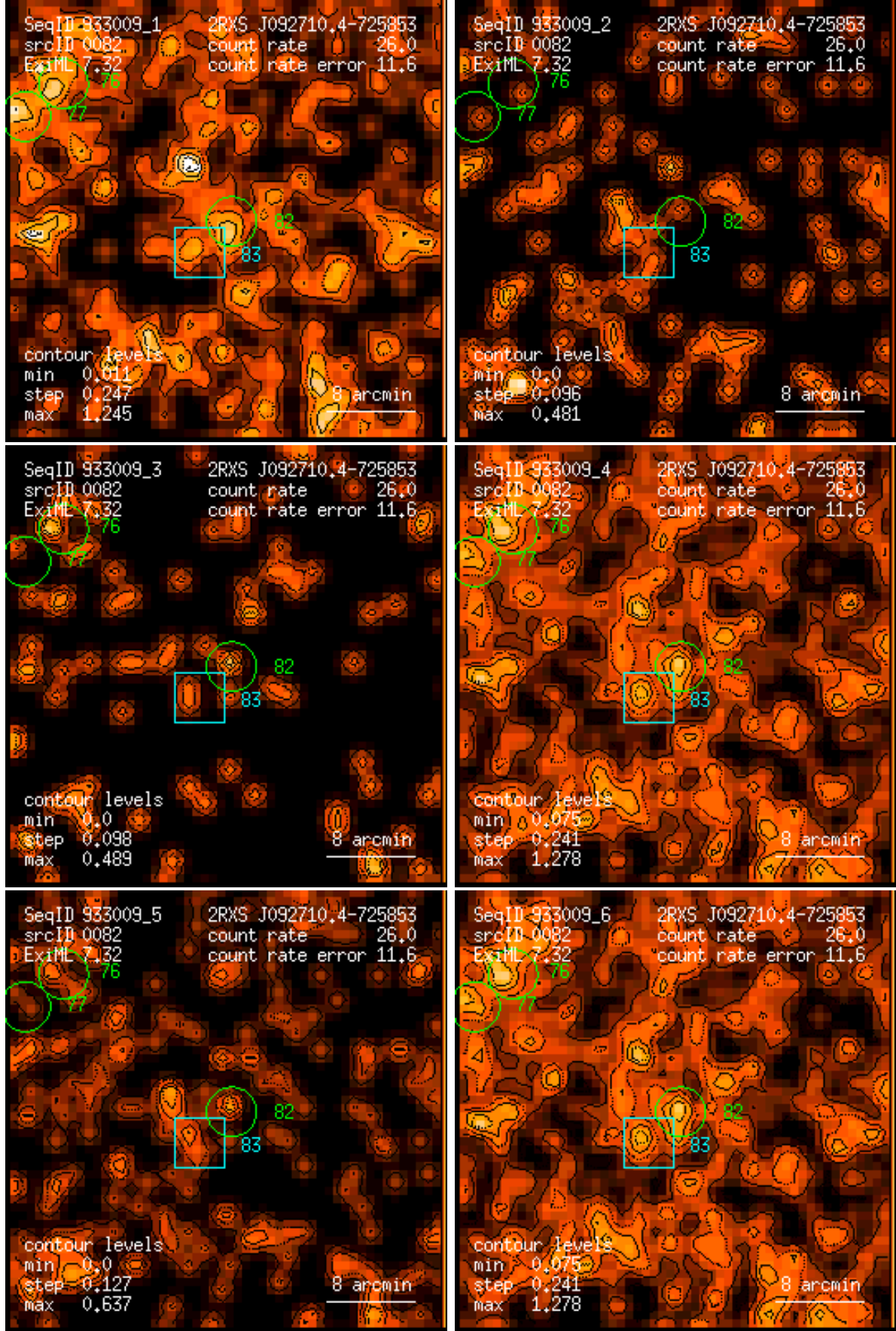
Figure 82: RASS 933009: detection 0082: band rate images, Gaussian filter: (1) PSPC channels 11 – 41, (2) 52 – 90, (3) 91 – 201, (4) 11 – 235, (5) 52 – 201, (6) 11 – 201. Broad band rates in counts/ks. Band rate contour levels in counts/ks/arcmin 2 .
