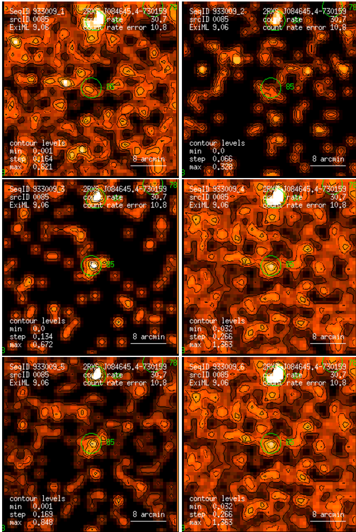
Figure 85: RASS 933009: detection 0085: band rate images, Gaussian filter: (1) PSPC channels 11 – 41, (2) 52 – 90, (3) 91 – 201, (4) 11 – 235, (5) 52 – 201, (6) 11 – 201. Broad band rates in counts/ks. Band rate contour levels in counts/ks/arcmin 2 .
