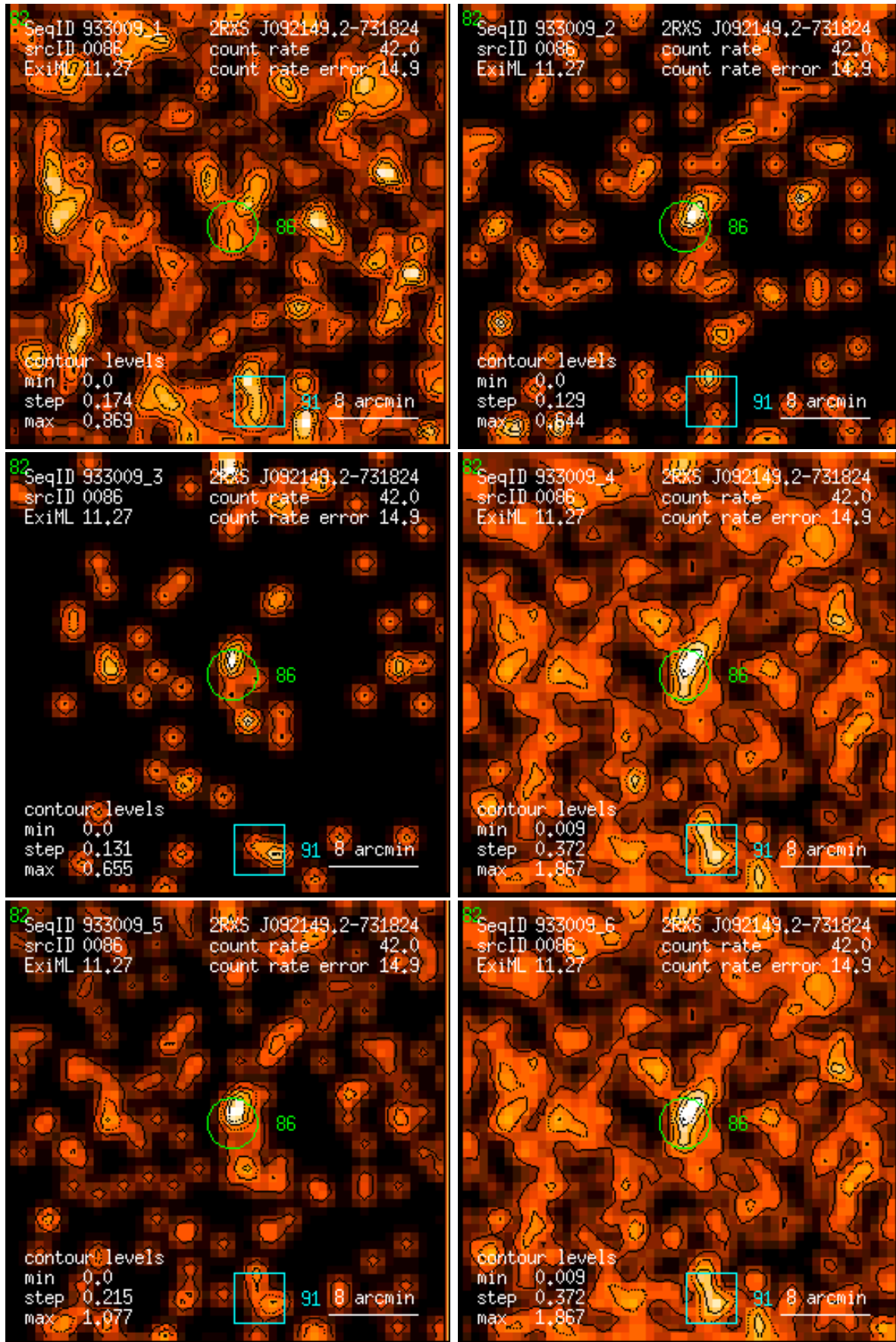
Figure 86: RASS 933009: detection 0086: band rate images, Gaussian filter: (1) PSPC channels 11 – 41, (2) 52 – 90, (3) 91 – 201, (4) 11 – 235, (5) 52 – 201, (6) 11 – 201. Broad band rates in counts/ks. Band rate contour levels in counts/ks/arcmin 2 .
