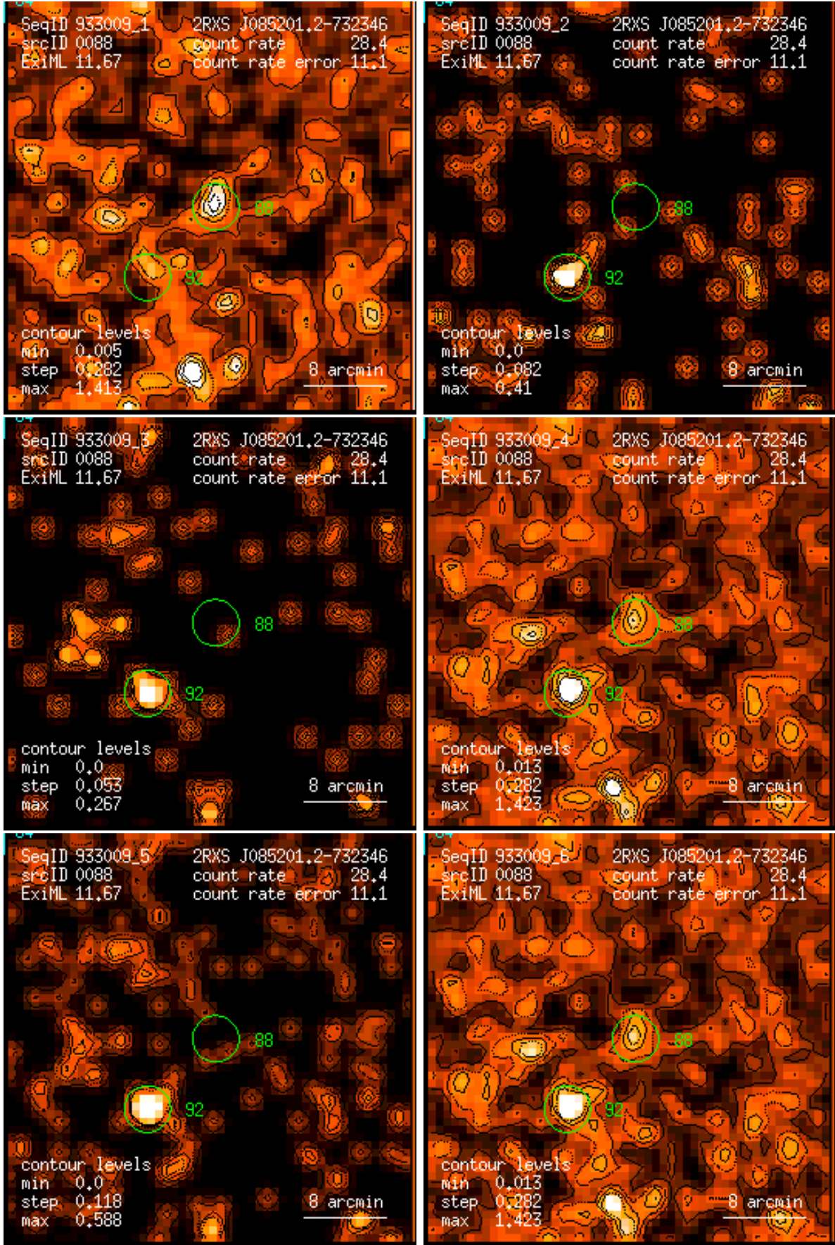
Figure 88: RASS 933009: detection 0088: band rate images, Gaussian filter: (1) PSPC channels 11 – 41, (2) 52 – 90, (3) 91 – 201, (4) 11 – 235, (5) 52 – 201, (6) 11 – 201. Broad band rates in counts/ks. Band rate contour levels in counts/ks/arcmin 2 .
