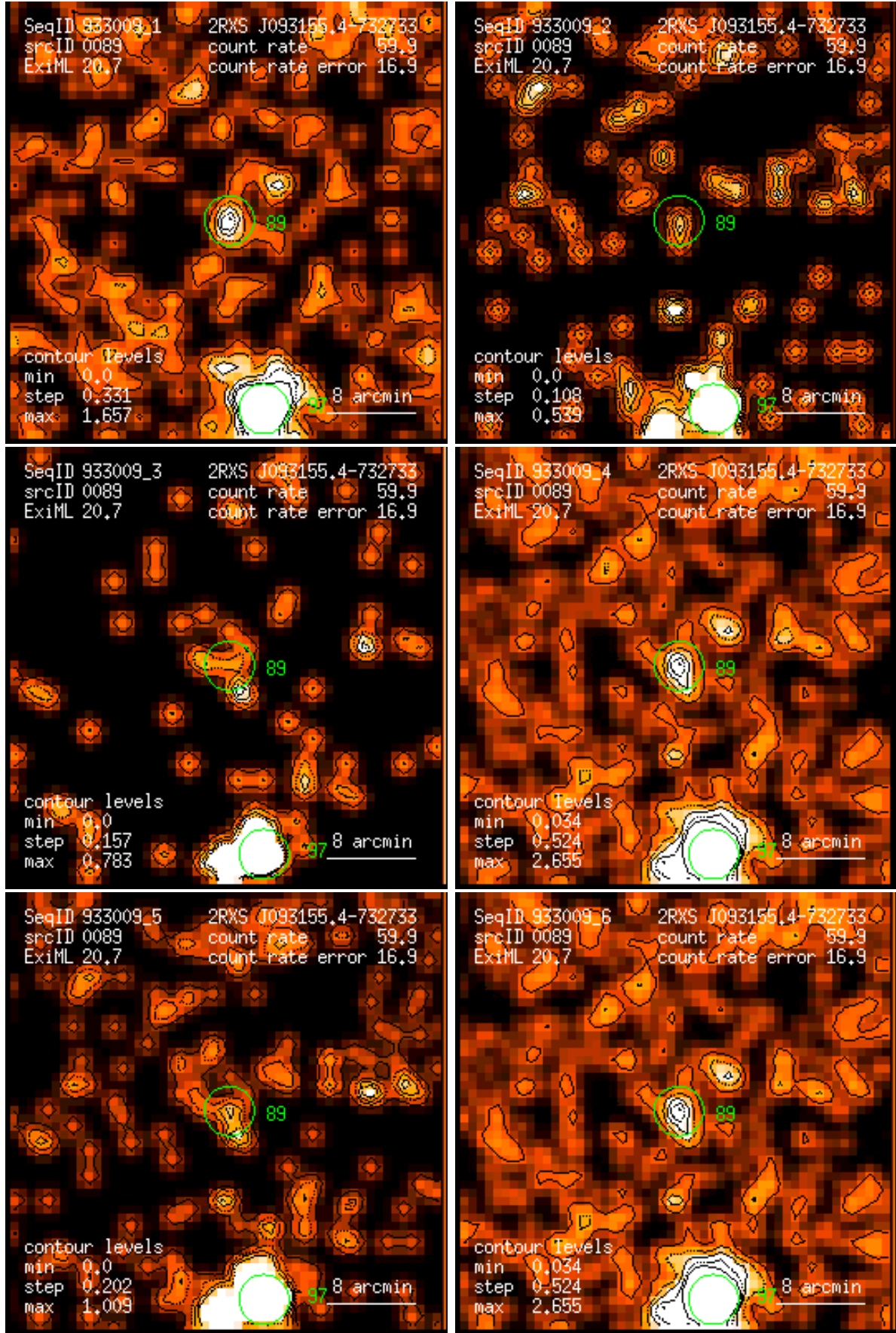
Figure 89: RASS 933009: detection 0089: band rate images, Gaussian filter: (1) PSPC channels 11 – 41, (2) 52 – 90, (3) 91 – 201, (4) 11 – 235, (5) 52 – 201, (6) 11 – 201. Broad band rates in counts/ks. Band rate contour levels in counts/ks/arcmin 2 .
