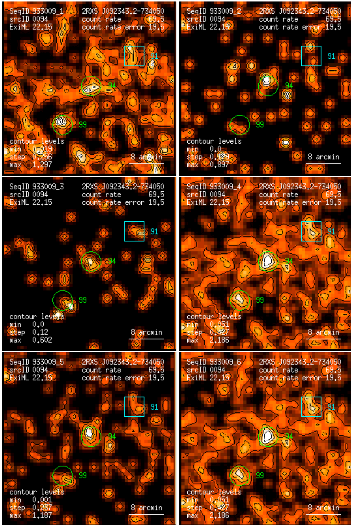
Figure 94: RASS 933009: detection 0094: band rate images, Gaussian filter: (1) PSPC channels 11 – 41, (2) 52 – 90, (3) 91 – 201, (4) 11 – 235, (5) 52 – 201, (6) 11 – 201. Broad band rates in counts/ks. Band rate contour levels in counts/ks/arcmin 2 .
